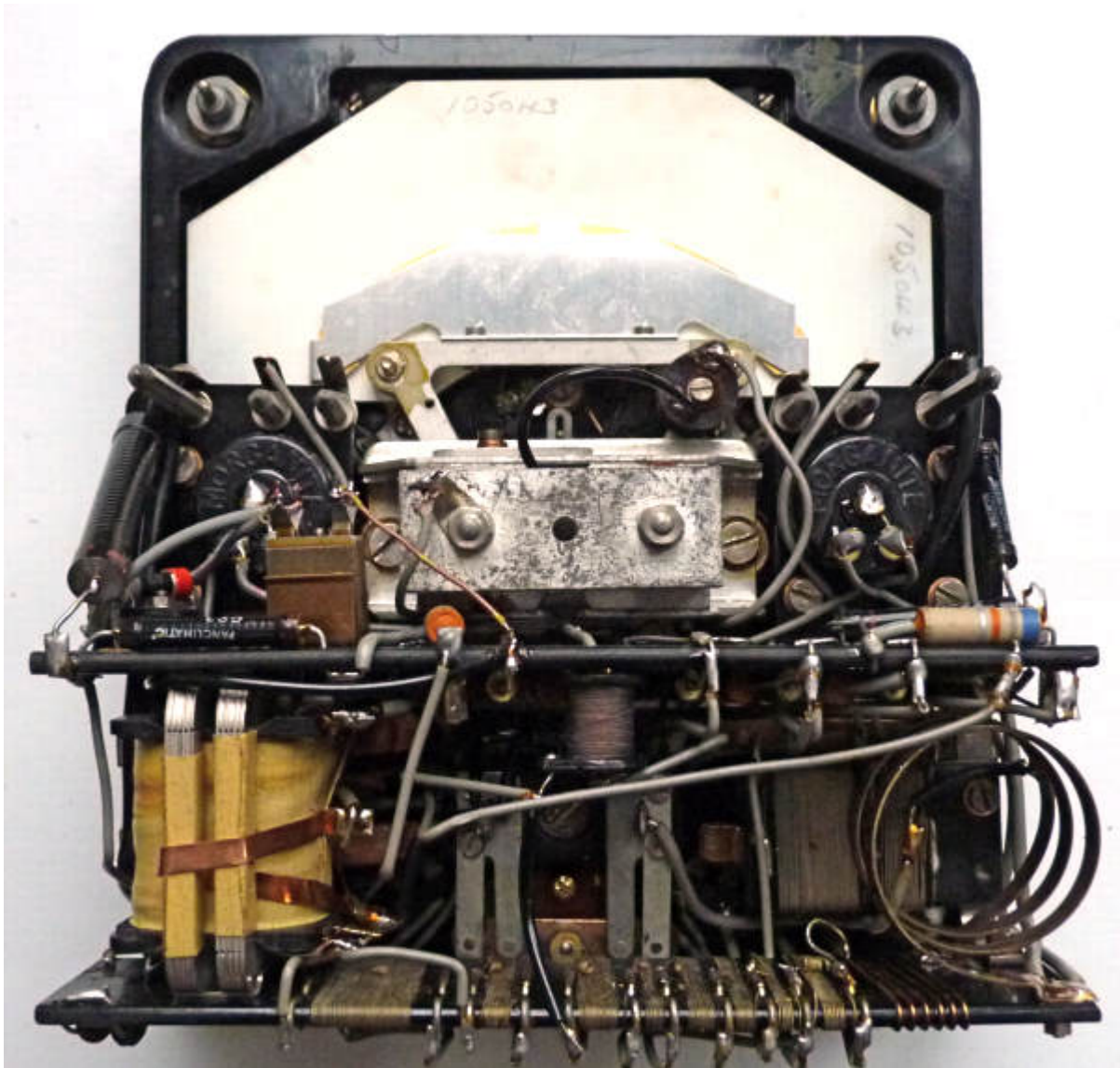
AVO Model8 MkII interior (the rectifier is not original)
