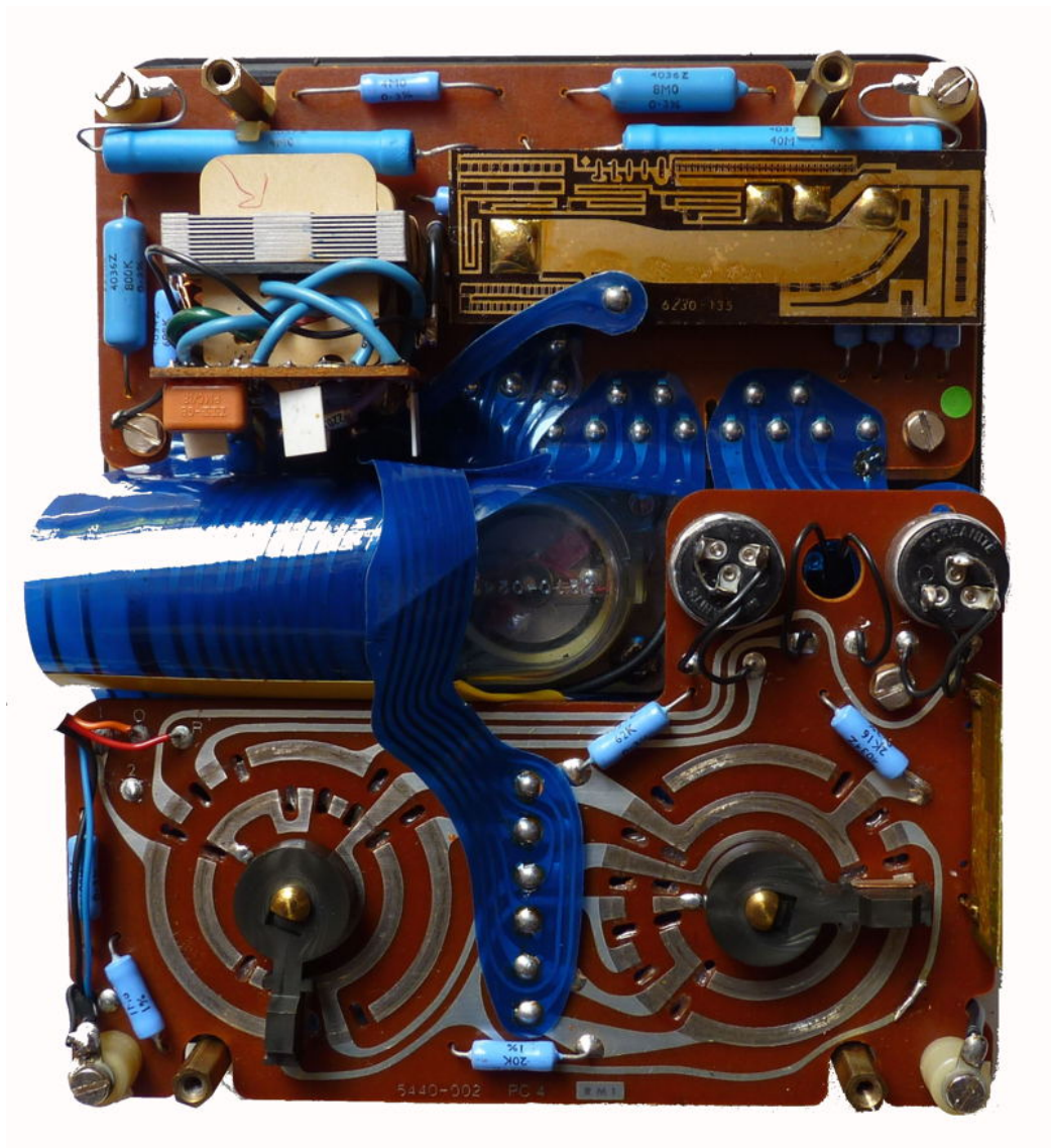
AVO Model8 MkV interior
