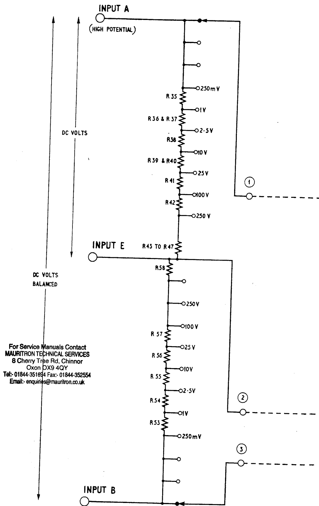
Fig.10. DC volts and DC volts (balanced) measuring circuit
