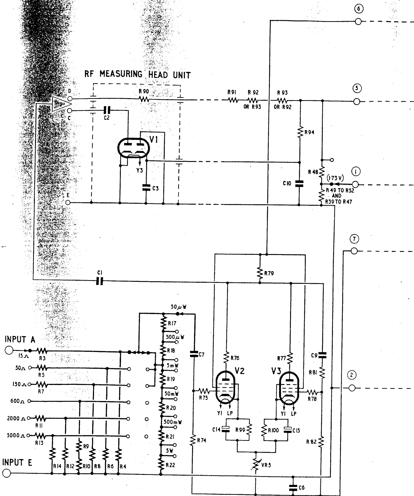
Fig.17.Watts measuring circuit
