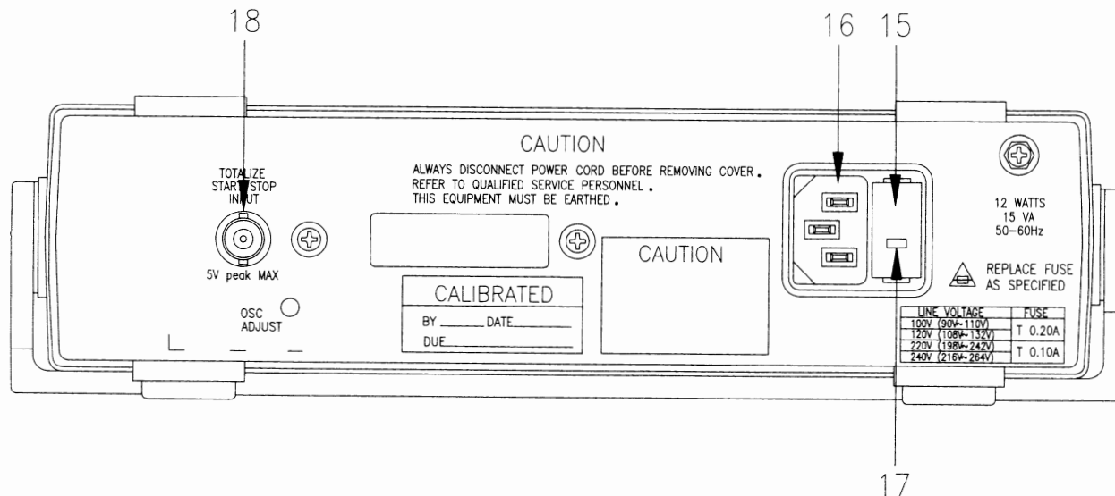
Figure 2-2 Rear Panel (100 MHz/crystal version)
