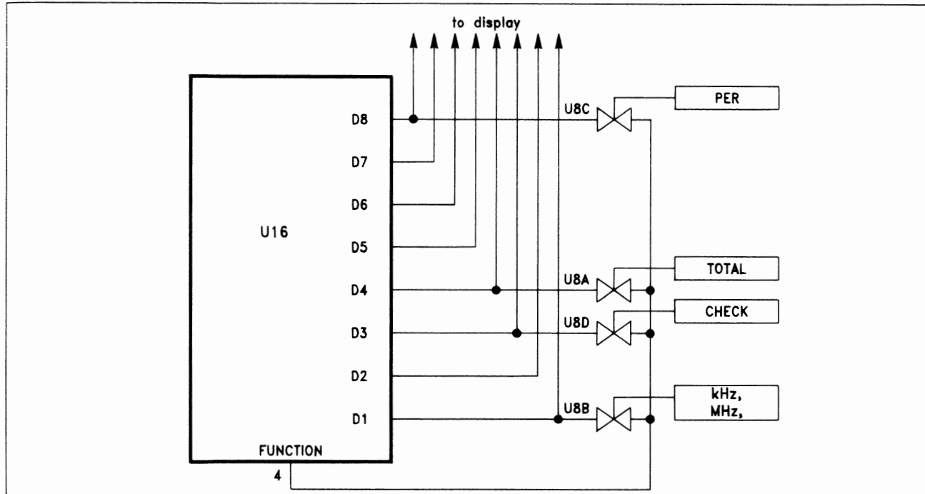
Figure 7-2. Function Selection 100 MHz
