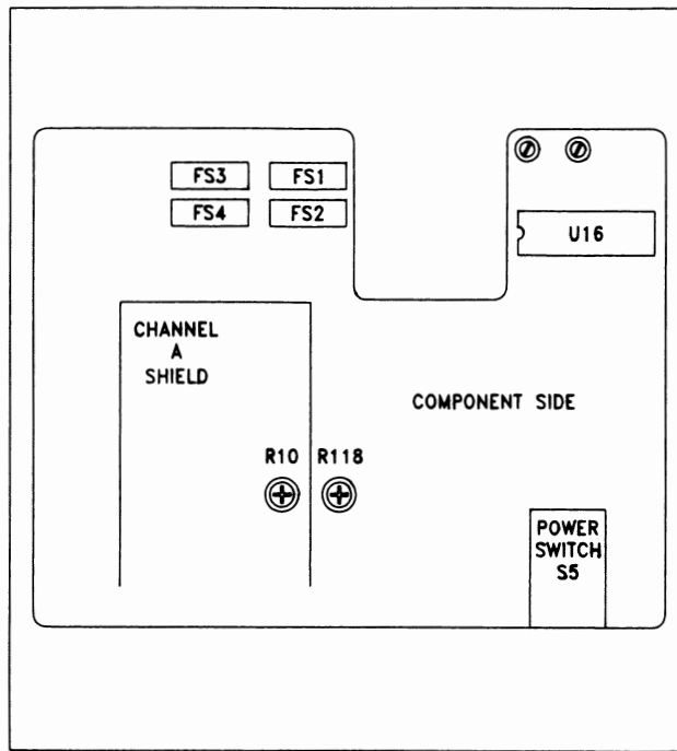
Figure 11-2. Main board Adjustments, Component Side View.
