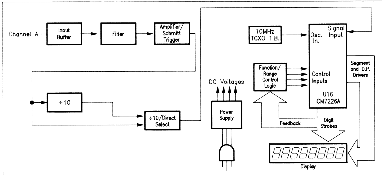
Figure 5-1. Block Diagram. 100 MHz (TCXO)
