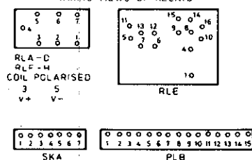
WIRING VIEWS OF RELAYS
