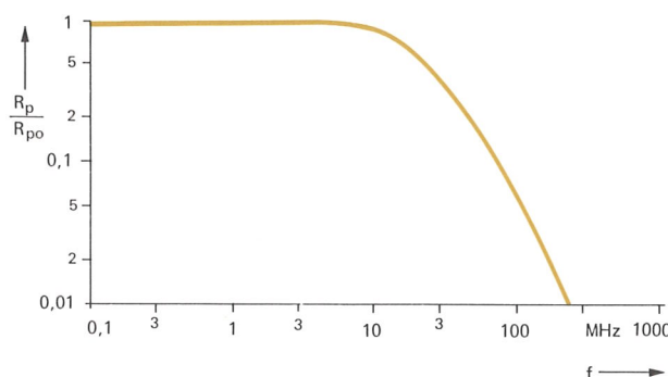
Typical frequency function of the input resistance R_p relative to the input resistance R_{po} at low frequencies.
