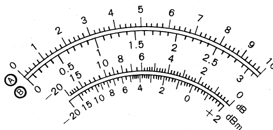
VOLTS DECIBELS 0 dBm = 1mW/600Ω
