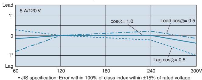
Voltage characteristic
