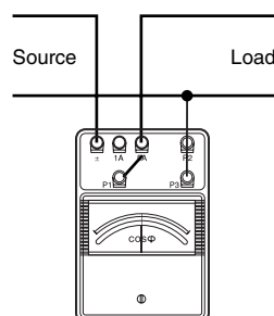
Single-phase circuit
