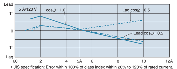
Current characteristic
