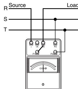
Balanced three-phase circuit
