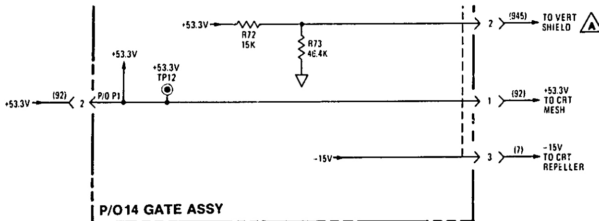
Figure 7-3. Changes to Schematic 17
