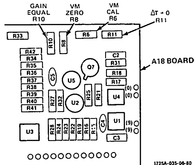
Figure 7-4. Analog Assembly Adjustments
