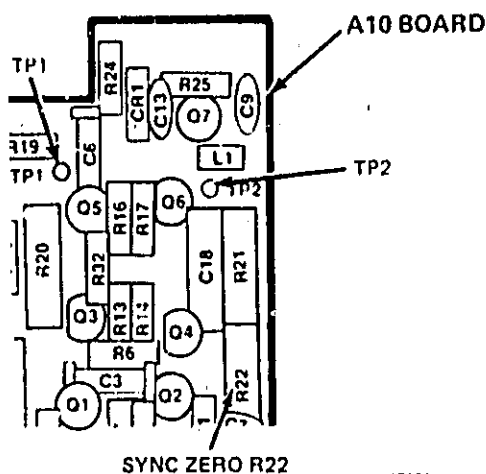
Figure 5-15. Sync Balance Adjustment
