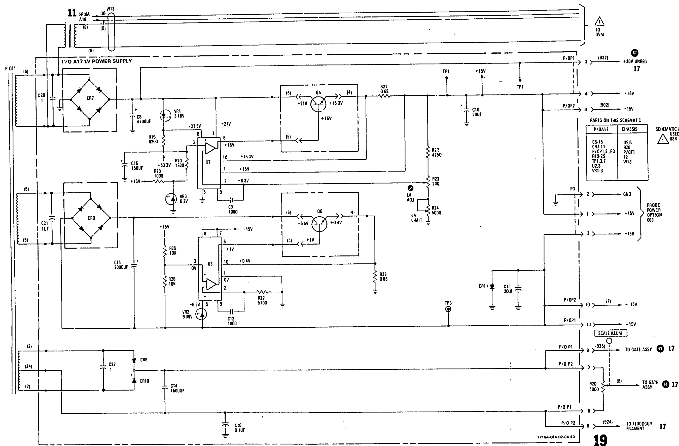
Figure 8-21. Service Information, Low-voltage Power Supply, Assembly A17 (Sheet 4 of 4) 8-51
