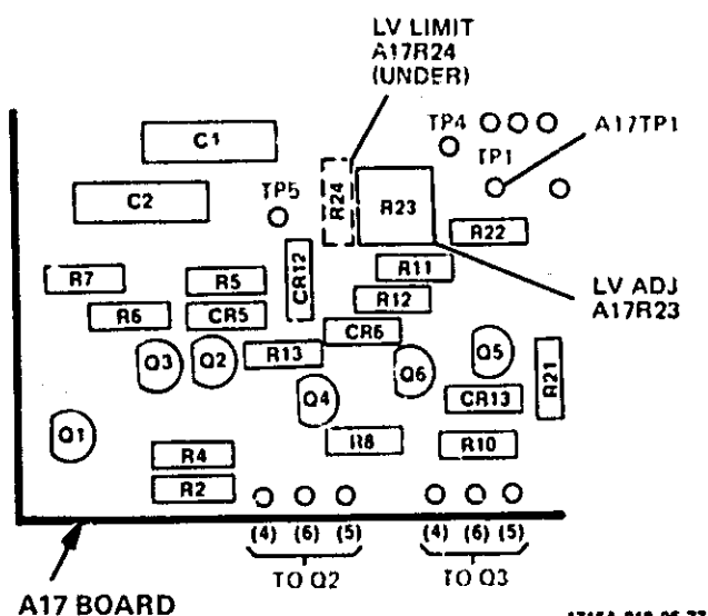
Figure 5-10. Low-voltage Power Supply Adjustment
