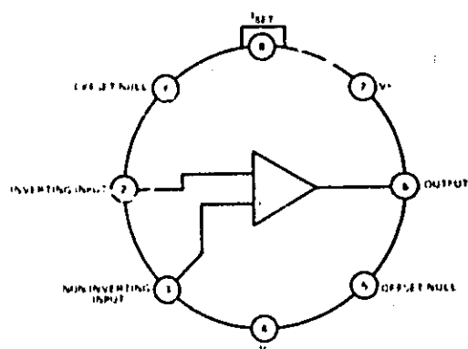
1826-0086 TOP VIEW
