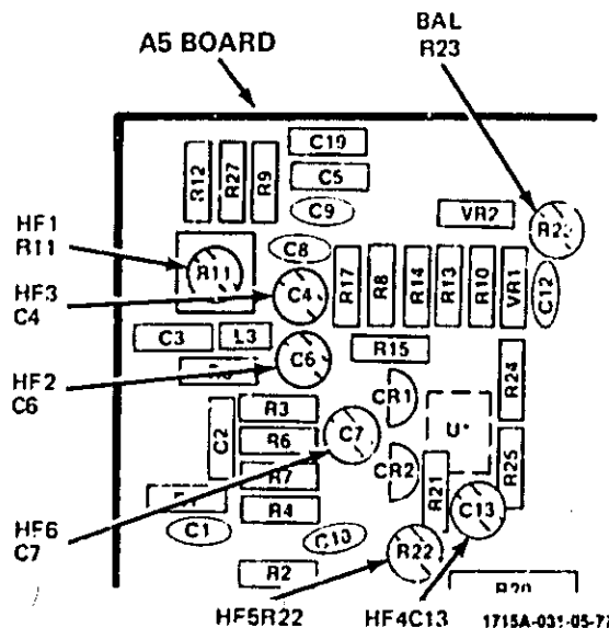
Figure 5-16. Vertical Output Amplifier Adjustments
