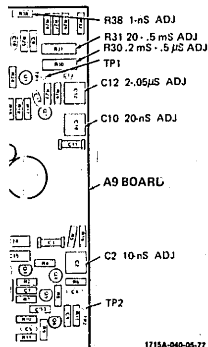
Figure 5-22. Delayed Sweep Adjustments
