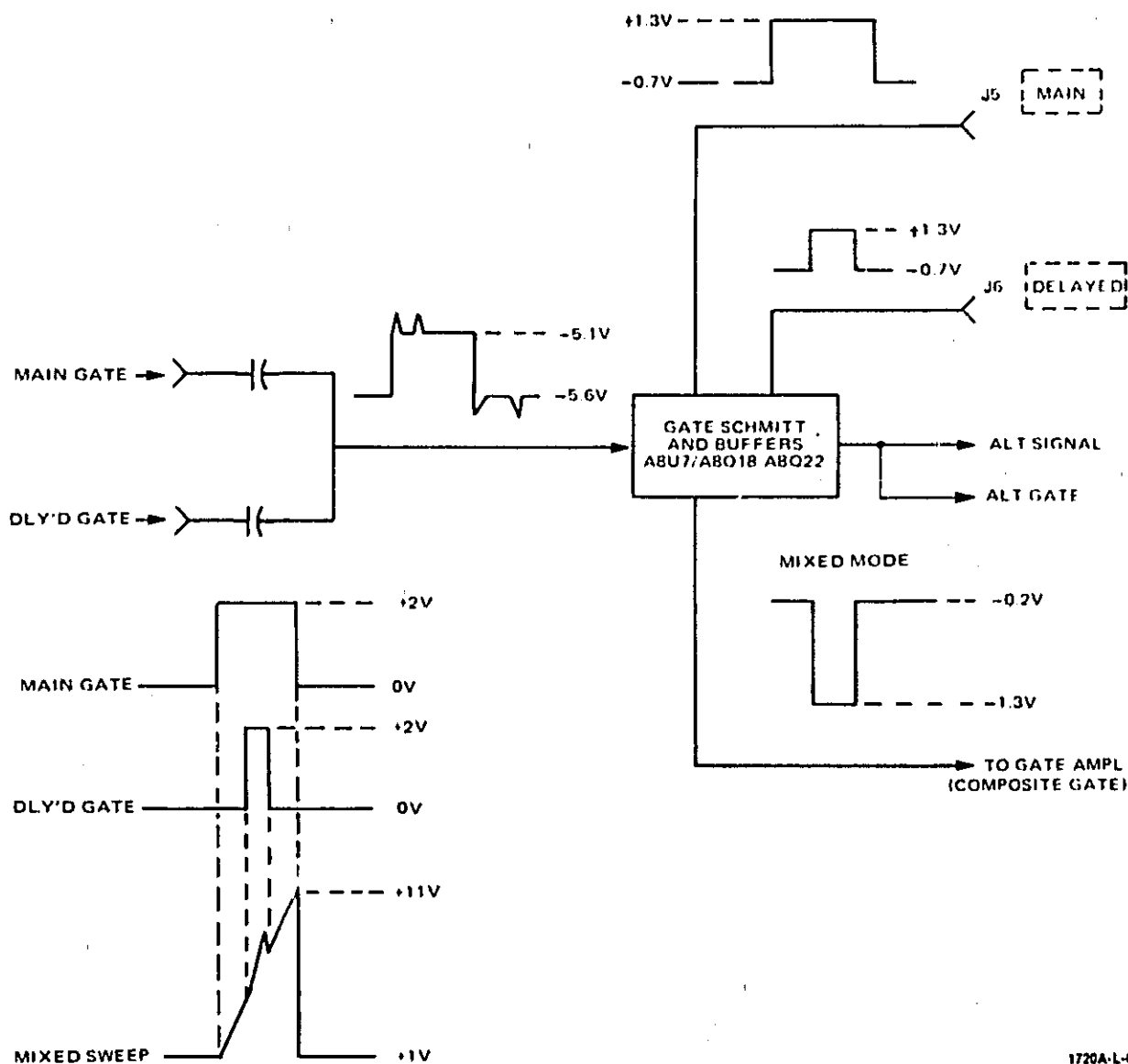
Figure 4-2. Schmitt Simplified Block Diagram (Mixed Mode)
