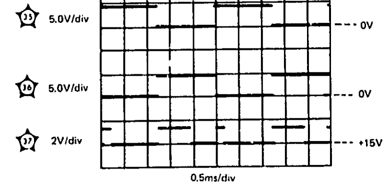
Figure 8-15. Service Information, Holdoff-delayed Comparator, Assembly A12 (Sheet 1 of 2)
