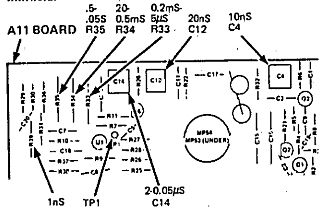
Figure 5-20. Main Sweep Adjustment
