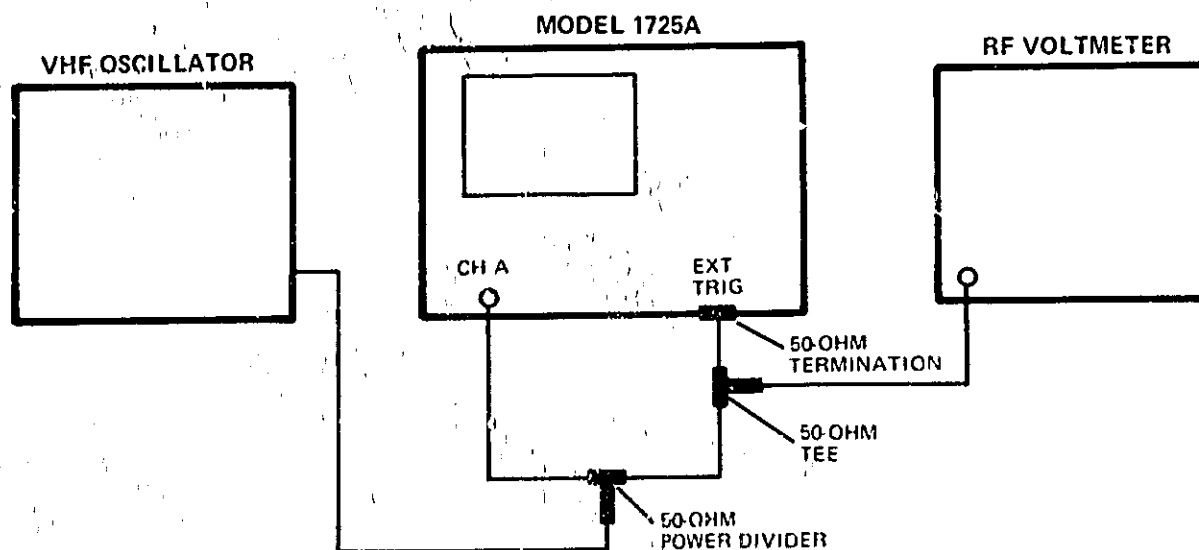
Figure 5-5. Main Triggering Test Setup
