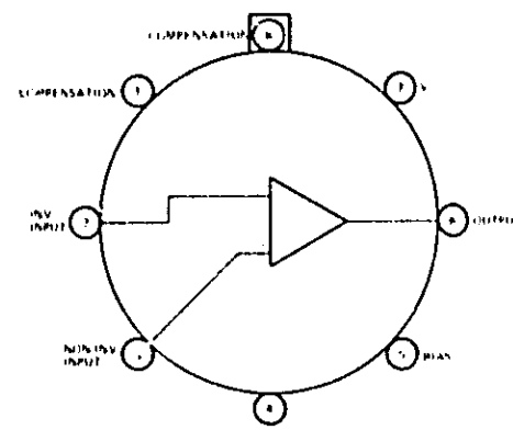
1826-0187 TOP VIEW
