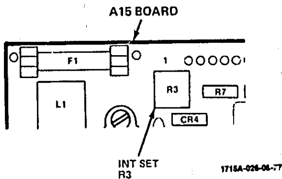
Figure 5-11. Intensity Adjustment
