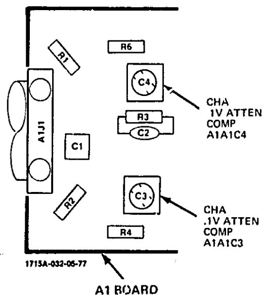
Figure 5-17. Attenuator Adjustments
