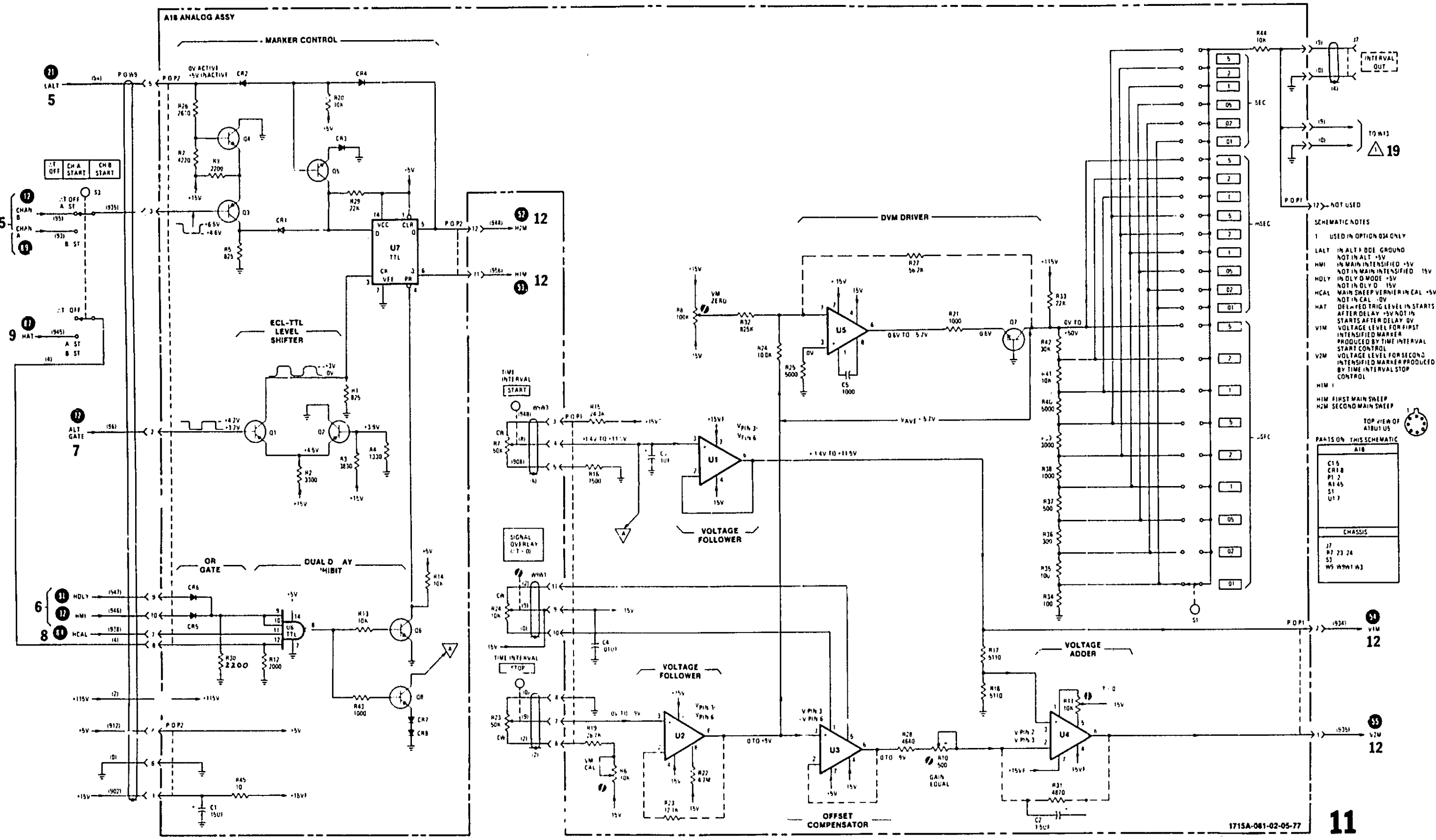
Figure 7-8. Replacement for Schematic 11 7-11/(7-12 blank)
