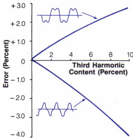
Theoretical error in the output of an average-responding converter, produced by third-harmonic distortion.
