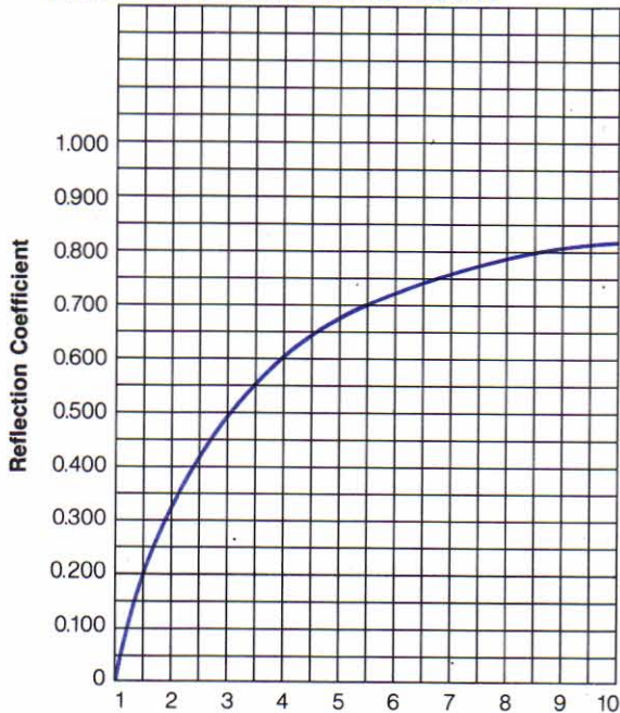
Reflection Coefficient vs. VSWR
