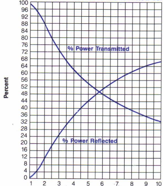
Power Reflected & Power Transmitted vs. VSWR
