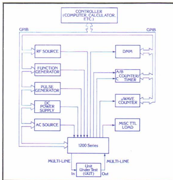
Figure 1 shows the block diagram of a typical system using the Series 1200.
