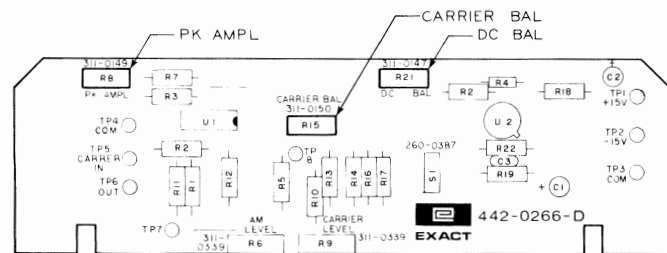
Fig. 5-4 Adjustment Locations
