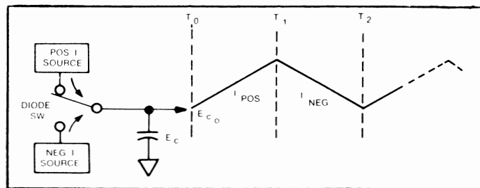
Fig. 4-1 Triangle Waveform
