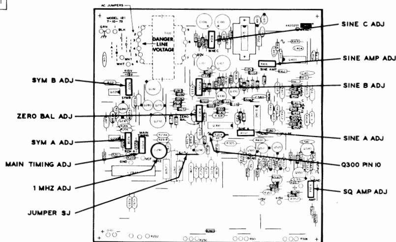
Fig. 5-4 Adjustment Locations
