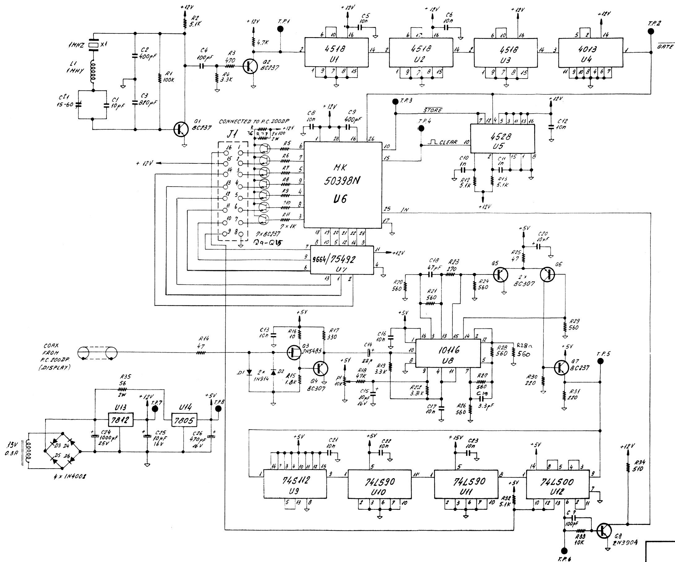
FIGURE 4-4. COUNTER PC 200C.
