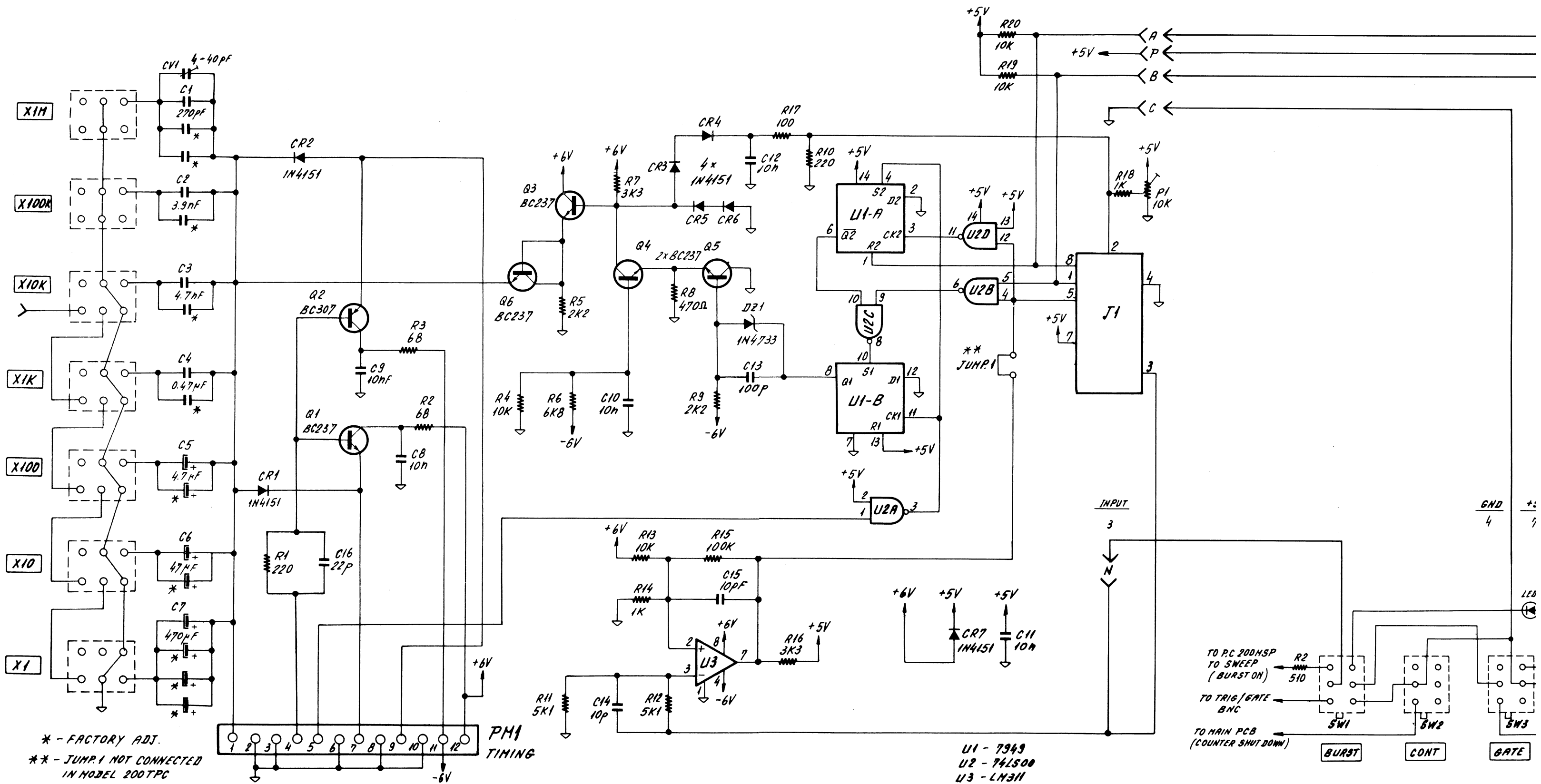
FIGURE 4-3. FREQUENCY RANGE SELECTOR
