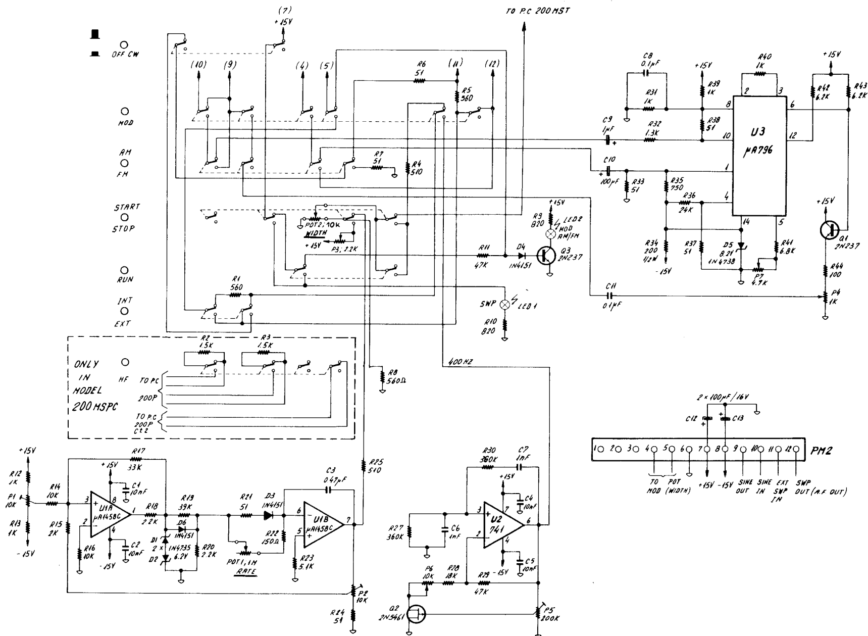
Figure 4-7. Sweep Generator PC200MSP, Schematic Diagram
