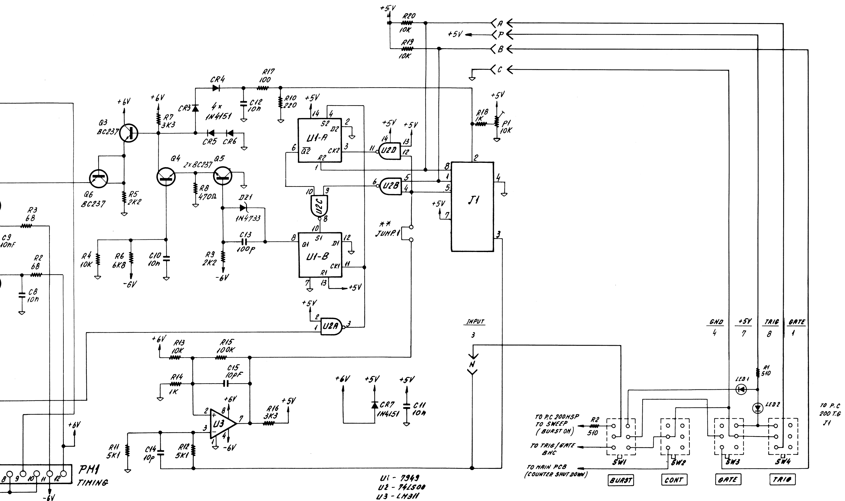
FIGURE 4-3. FREQUENCY RANGE SELECTOR PC 200TG.
