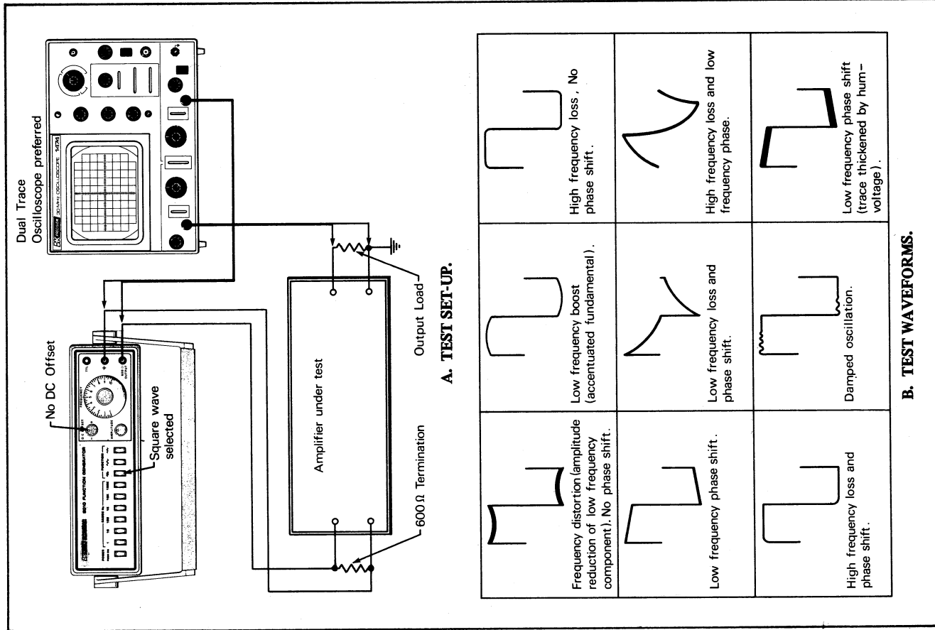
Fig. 9. Amplifier performance evaluation, using square waves.
