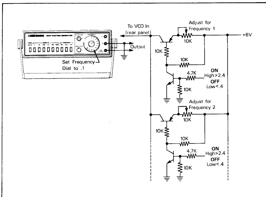
Fig. 14. Digitally programmed frequency selection.
