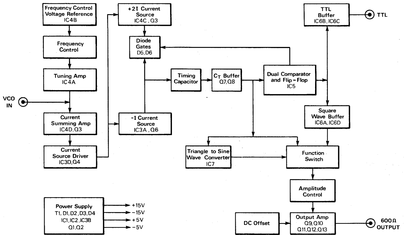
Fig. 16. Model 3010 block diagram.
