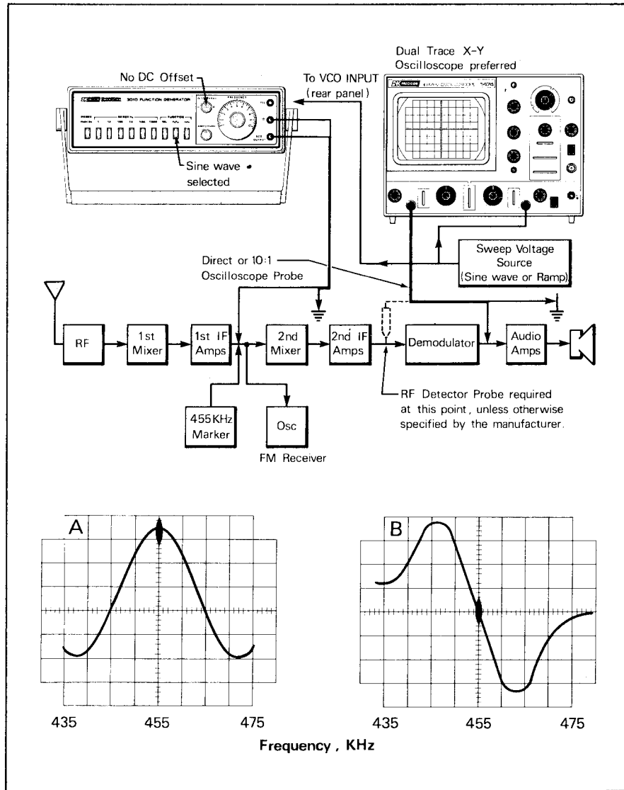
Fig. 15. Alignment of communications IF's and discriminators.
