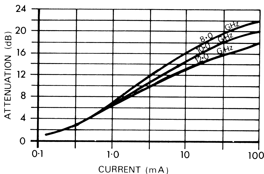
Fig. 5 Typical Modulator Performance
