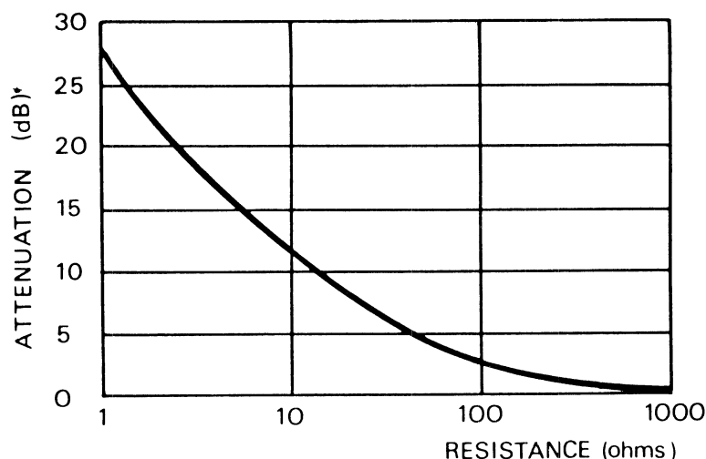
Fig. 7 Insertion Loss as a Function of Shunt Resistance in a 500 Line
