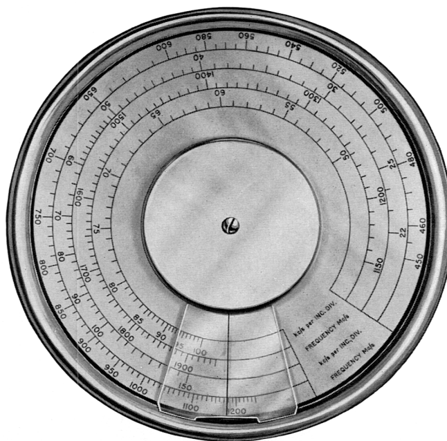
The large main tuning dial is directly calibrated in frequency and also shows the frequency change caused by turning the separate incremental dial through one division.
