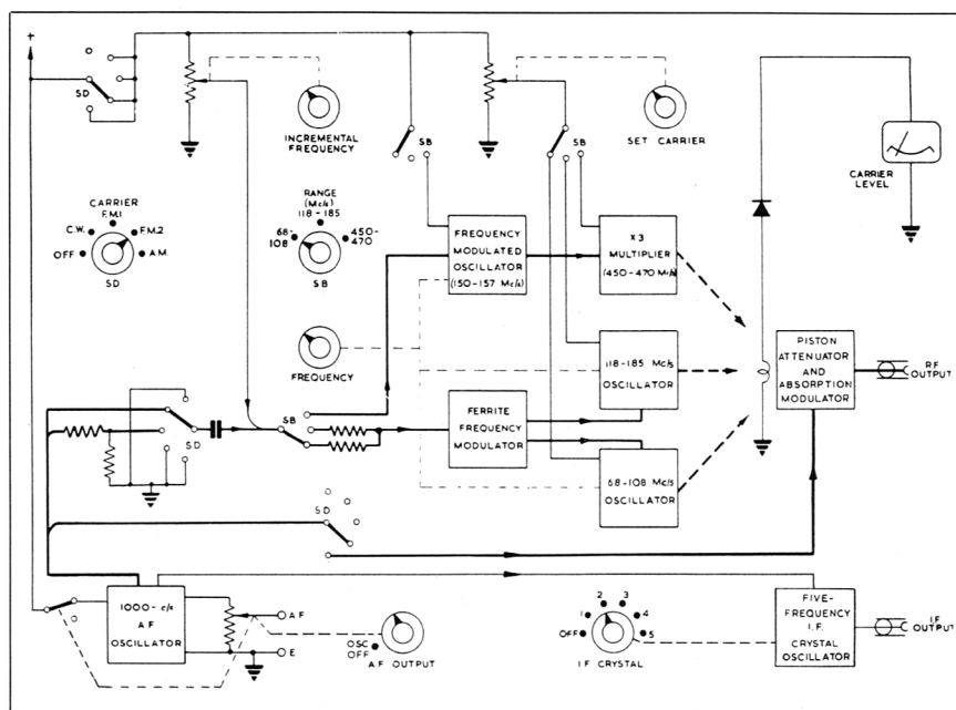
Functional Diagram of TF 1064A
