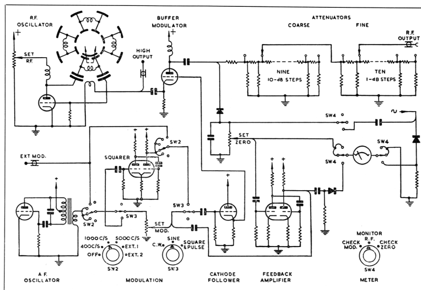
Functional Diagram of TF 801A/1
