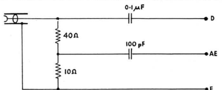
Circuit TM 6123
