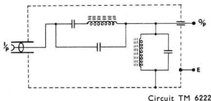
Circuit TM 6222
