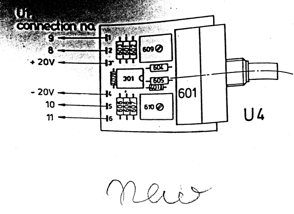
Fig. 35 Unit 4, component lay-out LO 06 onwards
