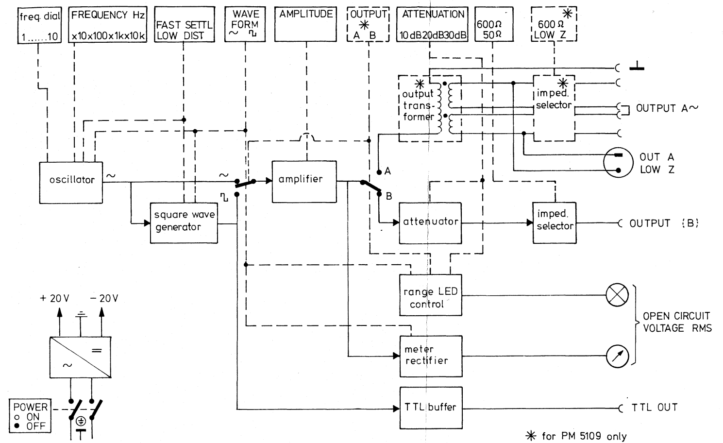
Fig. 30 Block diagram PM 5109/PM 5109 S
