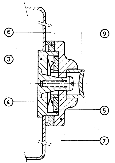
Fig. 36 Handle, spare parts
