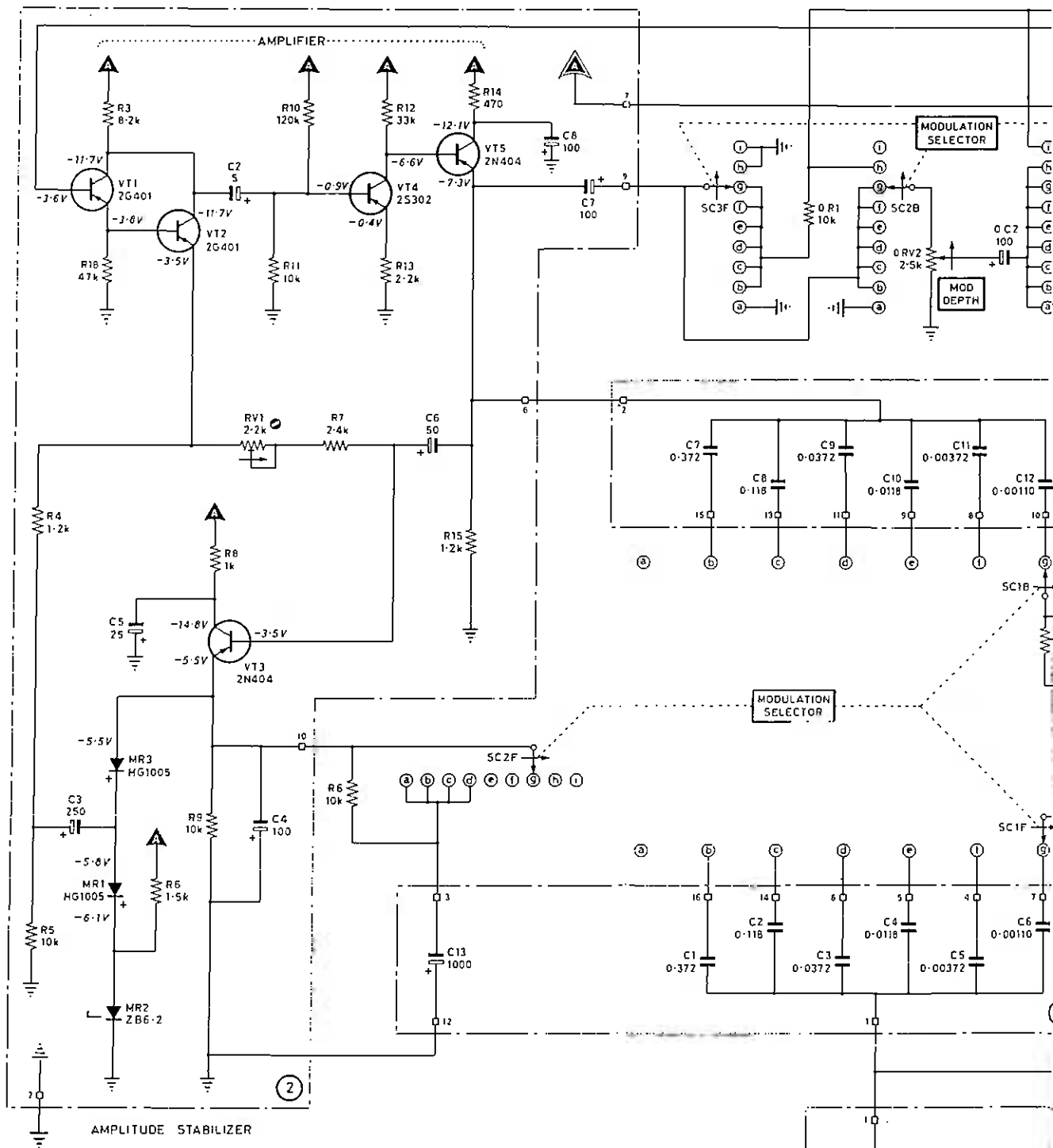
(2) and (29) MODULATION OSCILLATOR
