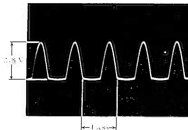
Fig. 4.13 Junction R30 and MR3, carrier frequency 1 Mc/s, carrier level meter set to 5 dB
