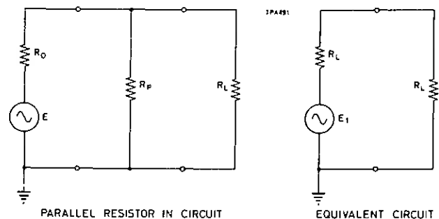
Fig. 2.9 Low-impedance matching
