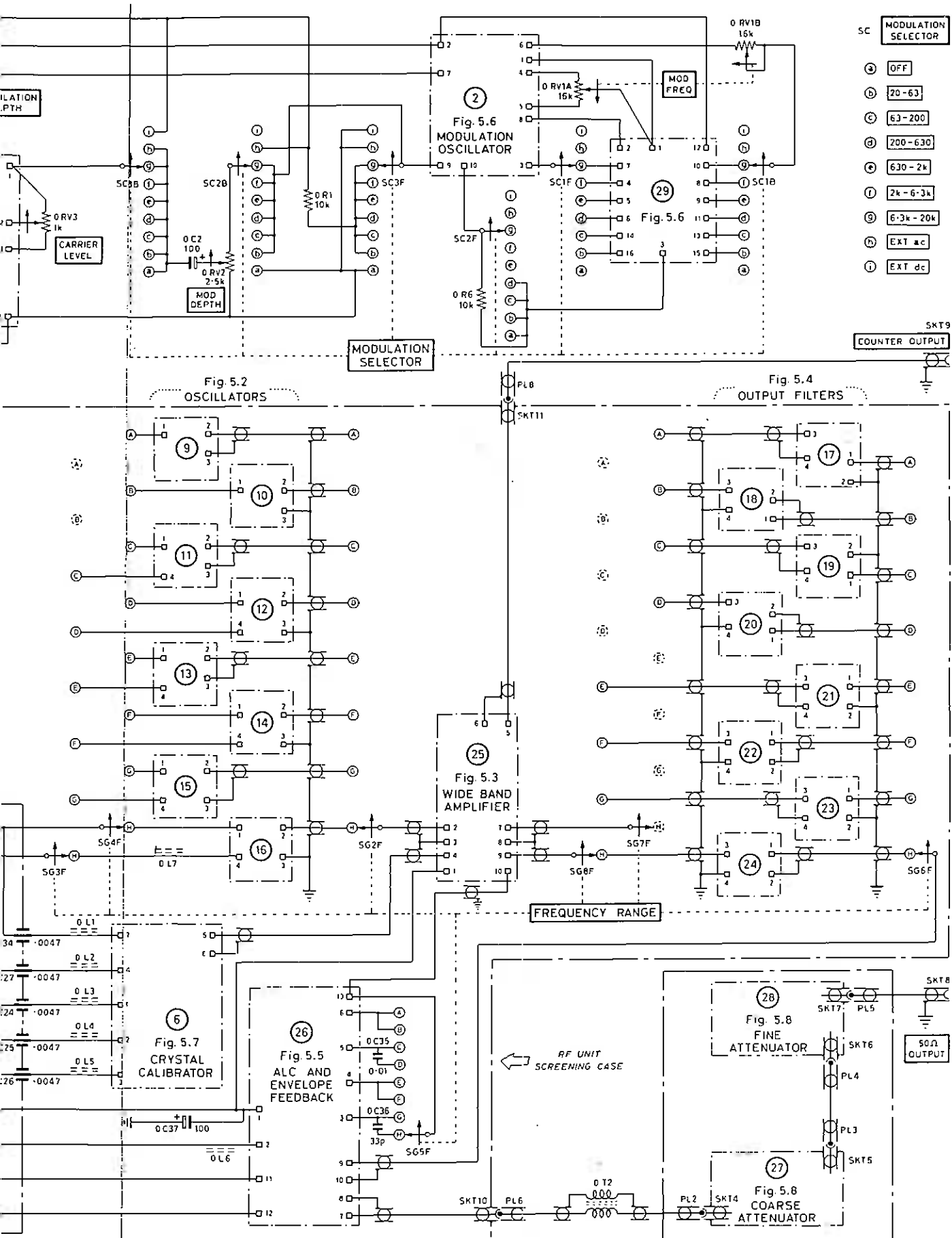
Fig. 5.1 Interconnection diagram
