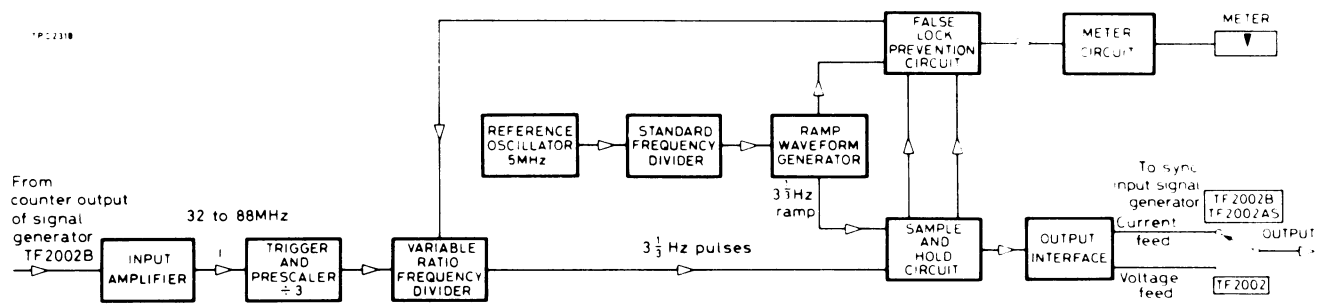
Fig. 3.2 Block diagram
