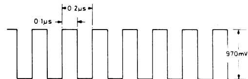
Fig. 4.13 Collector TR3, Schmitt trigger circuit
