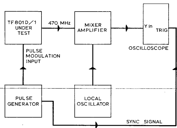
Fig. 1 Test gear arrangement for checking pulse modulation performance.
