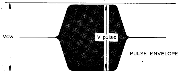
Fig. 2 Diagram of oscilloscope displays. Adjust attenuator to bring V_{\text{pulse}} equal to V_{\text{carrier}} . Attenuator movement should not exceed 2 dB.
