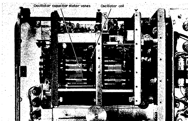
Rear view of R.F. box assembly with covers removed showing the oscillator capacitor stator vanes and the oscillator coil (range C). The 4 B.A. nuts may be slackened using a cranked spanner.
