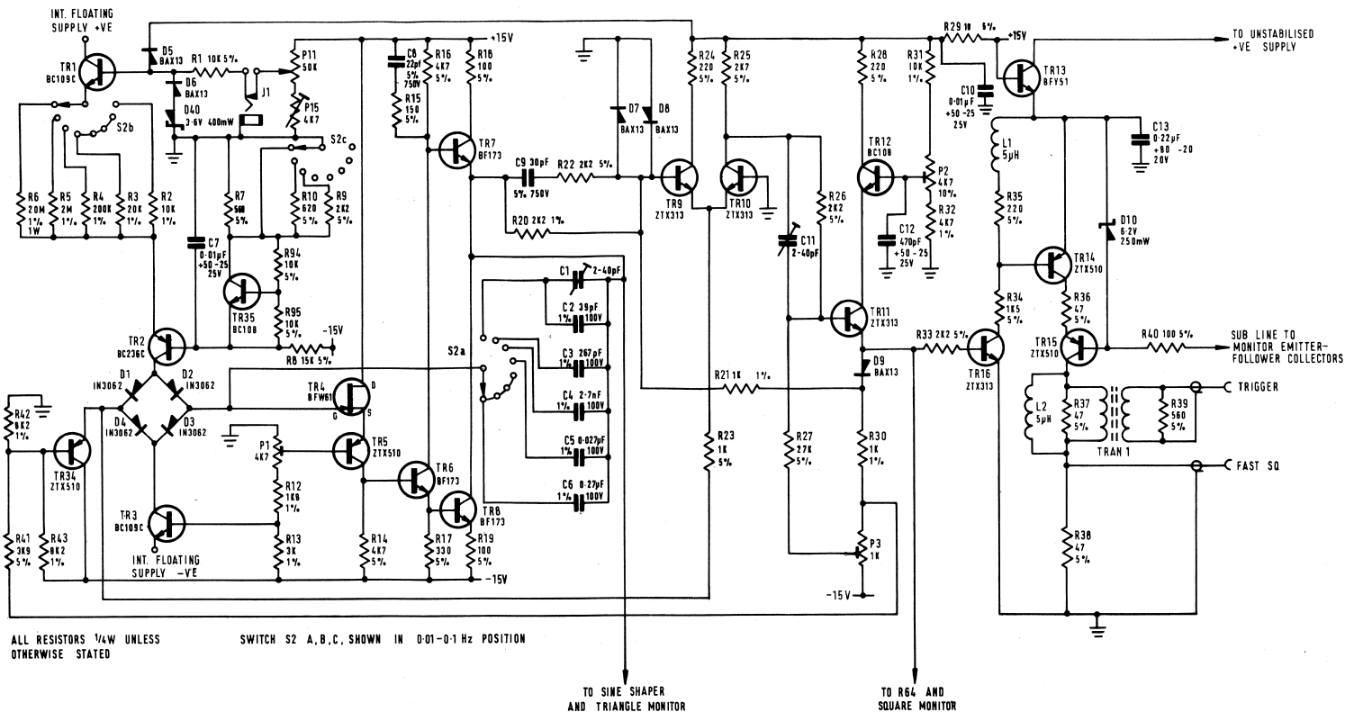
Fig 10 CIRCUIT DIAGRAM (Part 1)
