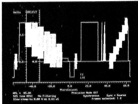
Vertical interval test signals can be seen very clearly for additional analysis of the signal. These can be printed as support documentation for automatic measurement results.
