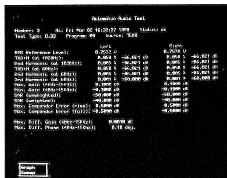
Automated audio measurement results.
