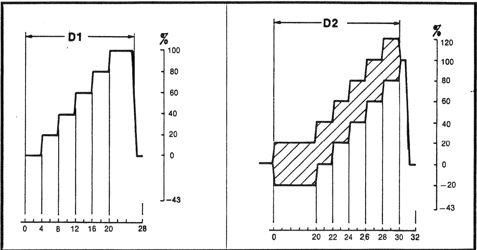
Elements D1 and D2 (CCIR Recommendation 569).
