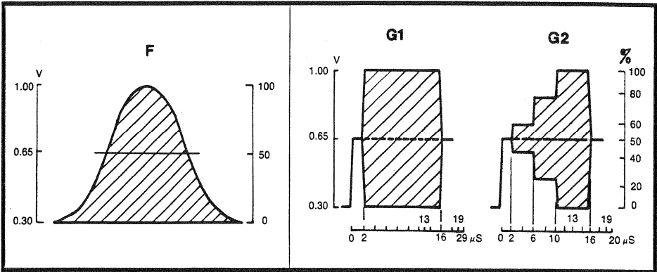
Elements F, G1, and G2 (CCIR Recommendation 567).
