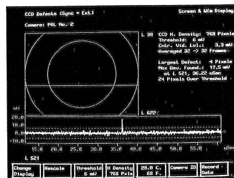
CCD Defects measurement with single-line waveform display.
