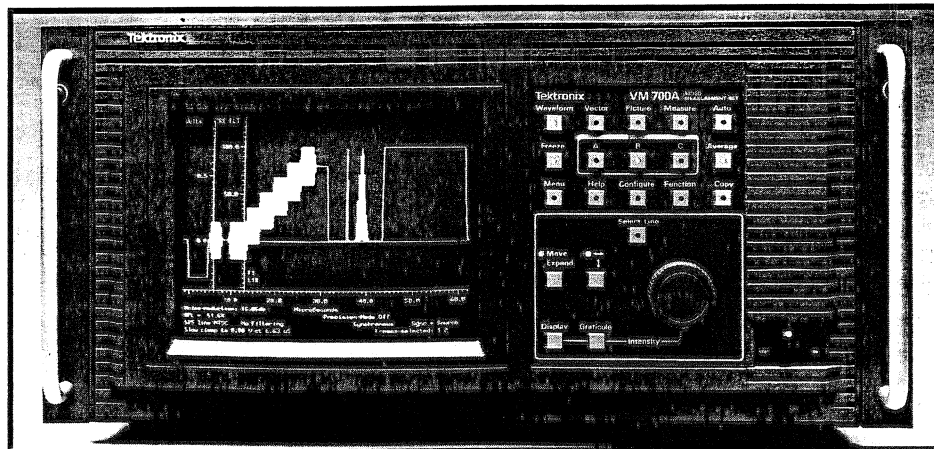
VM 700A Option 01 NTSC Video Measurement Set.
