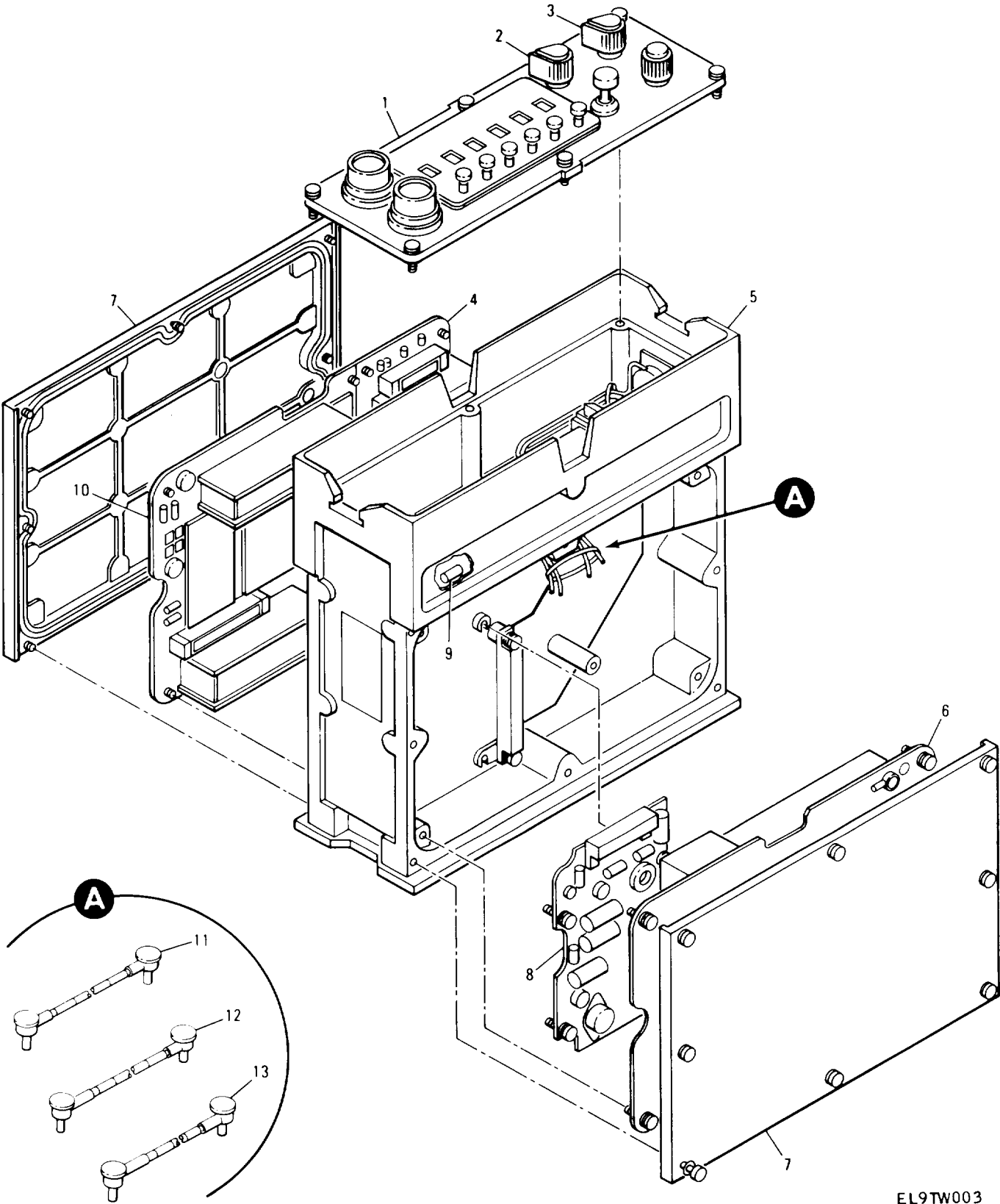
Figure 3. Receiver/Transmitter, RT-1209/URC
