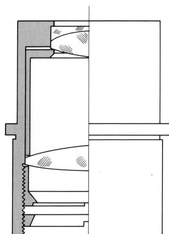
G10 \times Eyepiece
