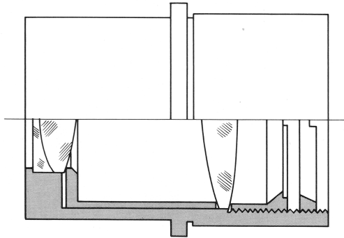
G10× Eyepiece
