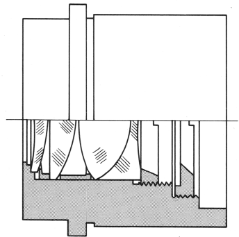
G20× Eyepiece
