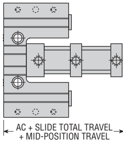
3 POSITION DETAIL
