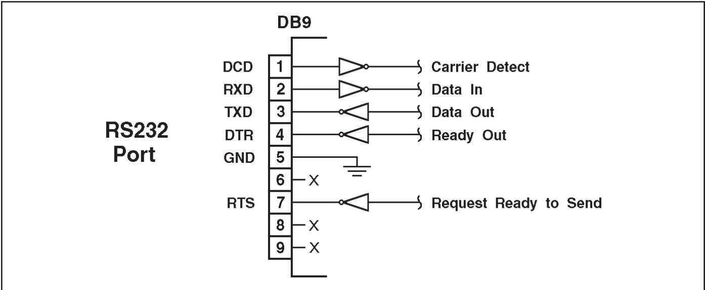
Figure A.2: Modem Port Interface
