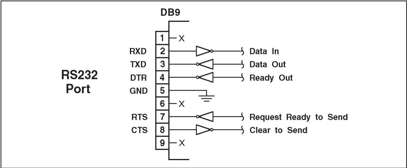
Figure A.1: Console Port Interface
