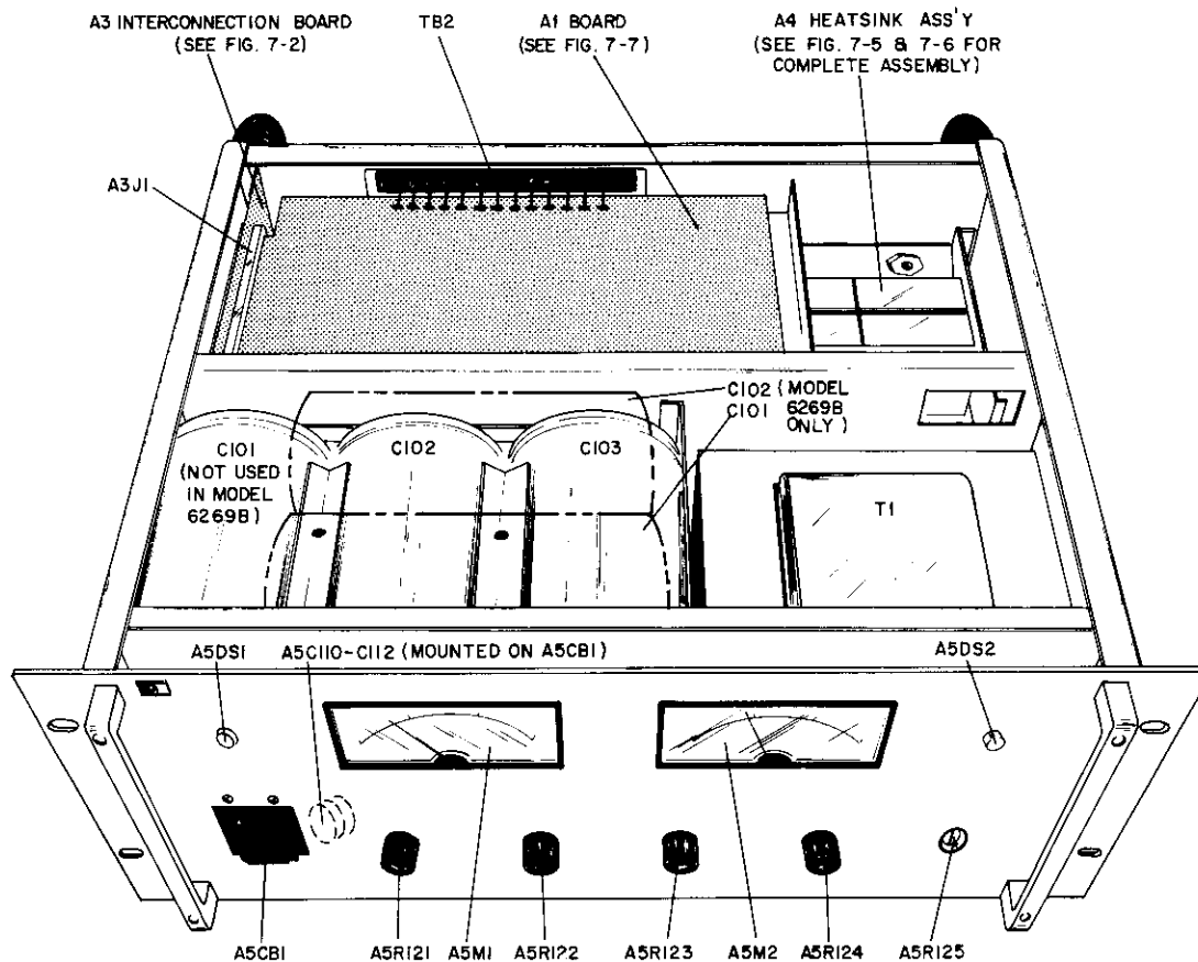
Figure 7-3. Chassis Component Locations, Top View
