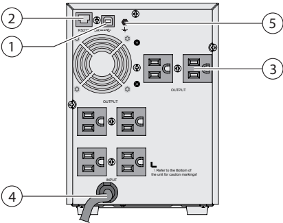
HP T1500 G4 NA/JP UPS
