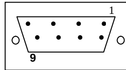
RS-232 pin definition
