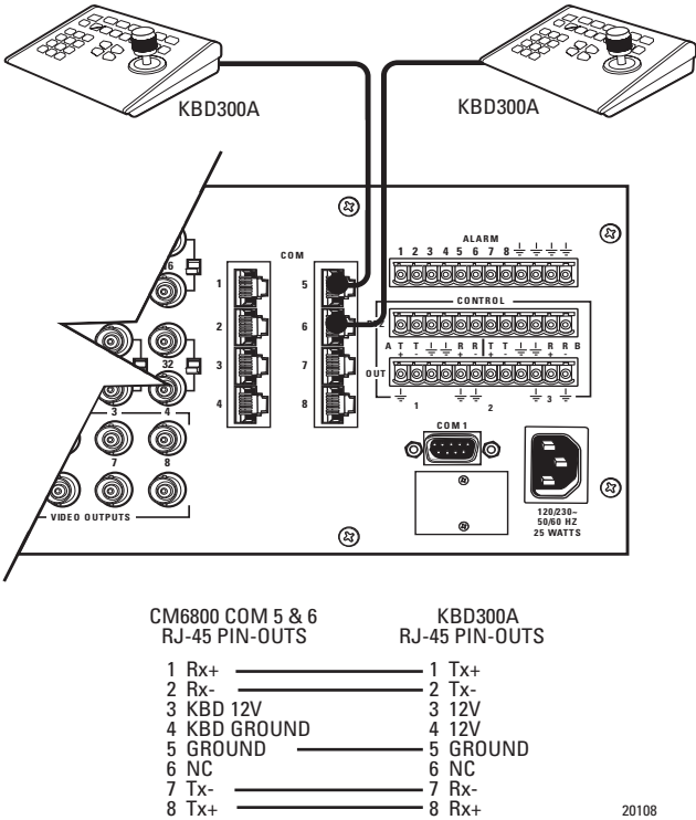
Figure 3. Data Cables Plugged into COM 5 and 6 (CM6800-48X8 Shown)
