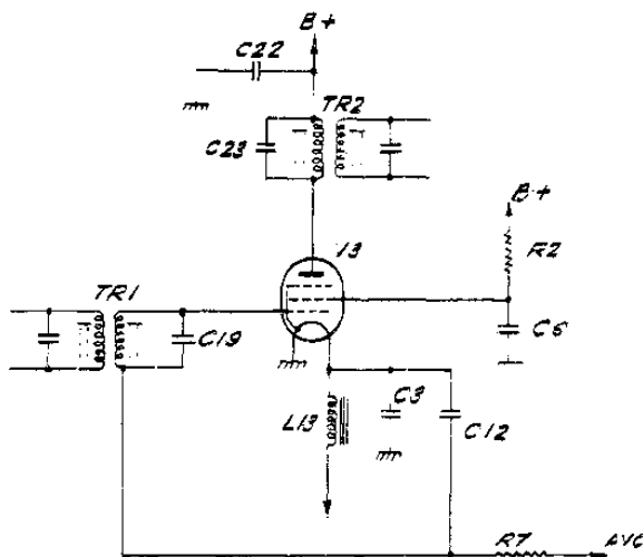
FIG. 7 - RECEIVER 1ST I.F. STAGE
