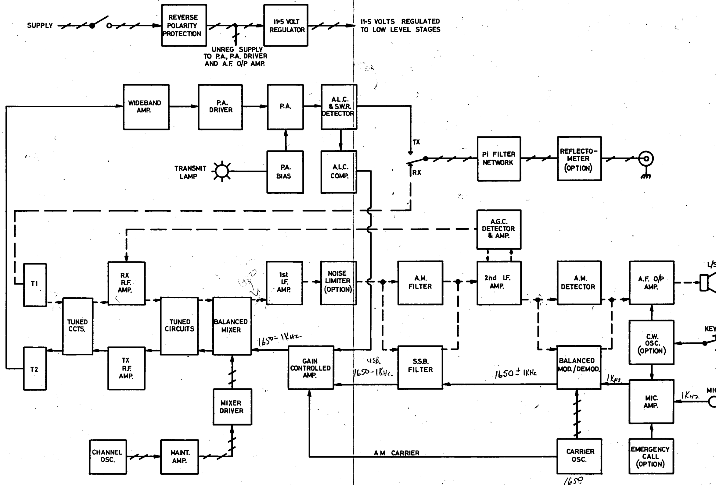
2. SIGNAL PATH BLOCK DIAGRAM
