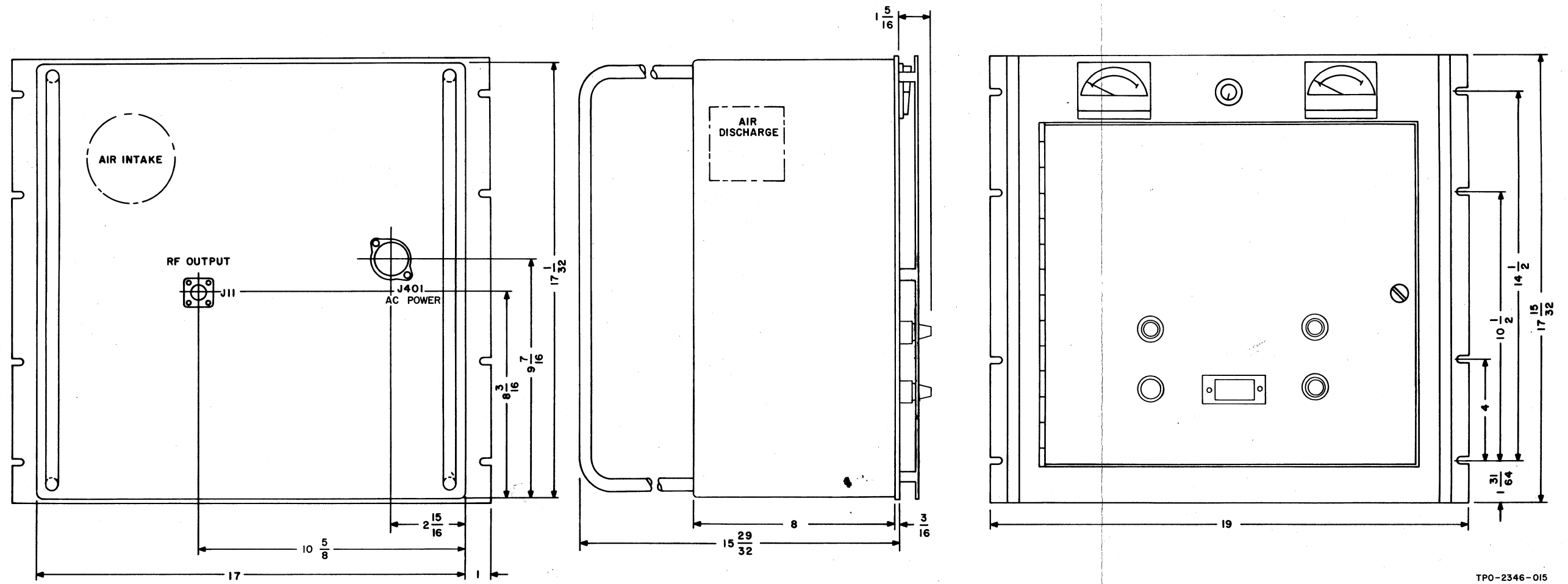
Figure 2-3. 242F-9C VHF/UHF Transmitter, Outline and Mounting Dimensions.
