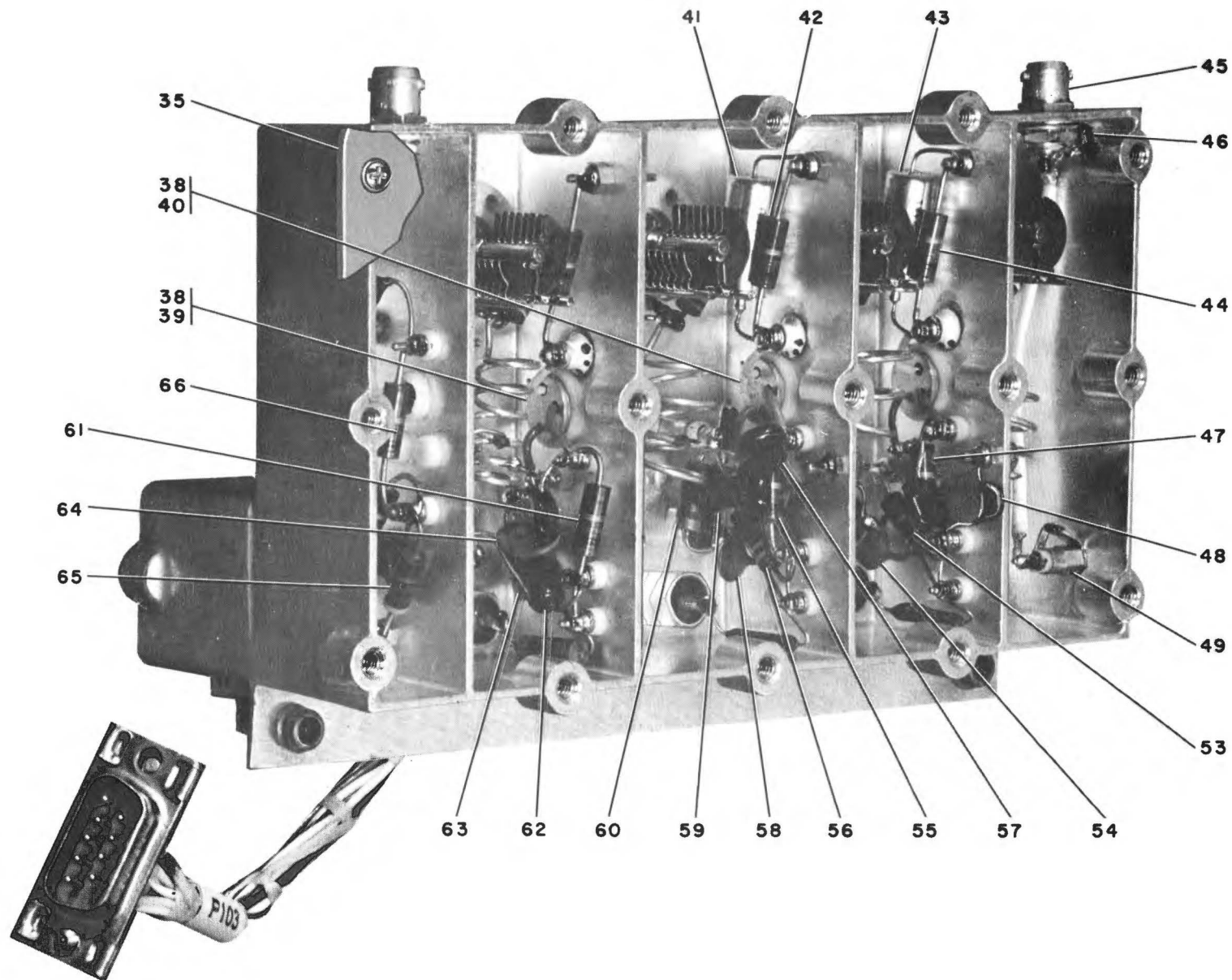
Figure 6-7. Transmitter VHF Exciter Subassembly (Sheet 2 of 4, Index 35 Through 66)
