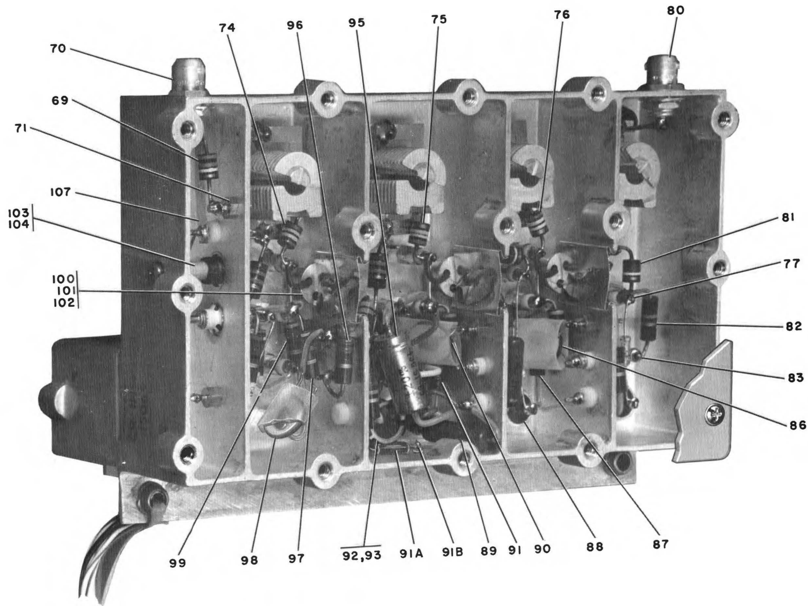
Figure 6-8. Transmitter UHF Exciter Subassembly (Sheet 3 of 4, Index 69 Through 107)
