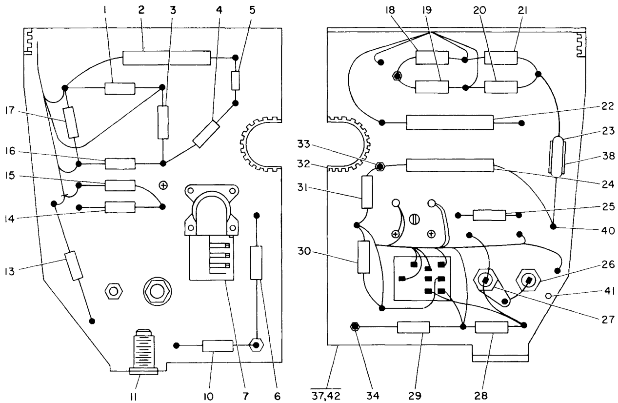
Figure 6-3. Electrical Component Bracket
