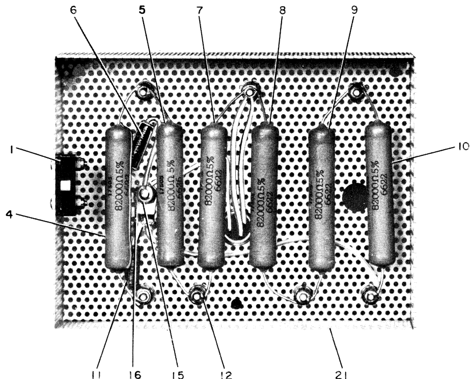
Figure 6-10. Resistor Assembly
