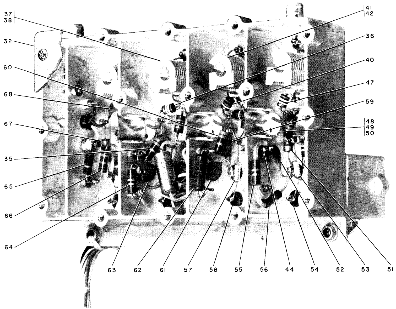
Figure 6-8. Transmitter UHF Exciter Subassembly (Sheet 2 of 4, Index 32 Through 68)
