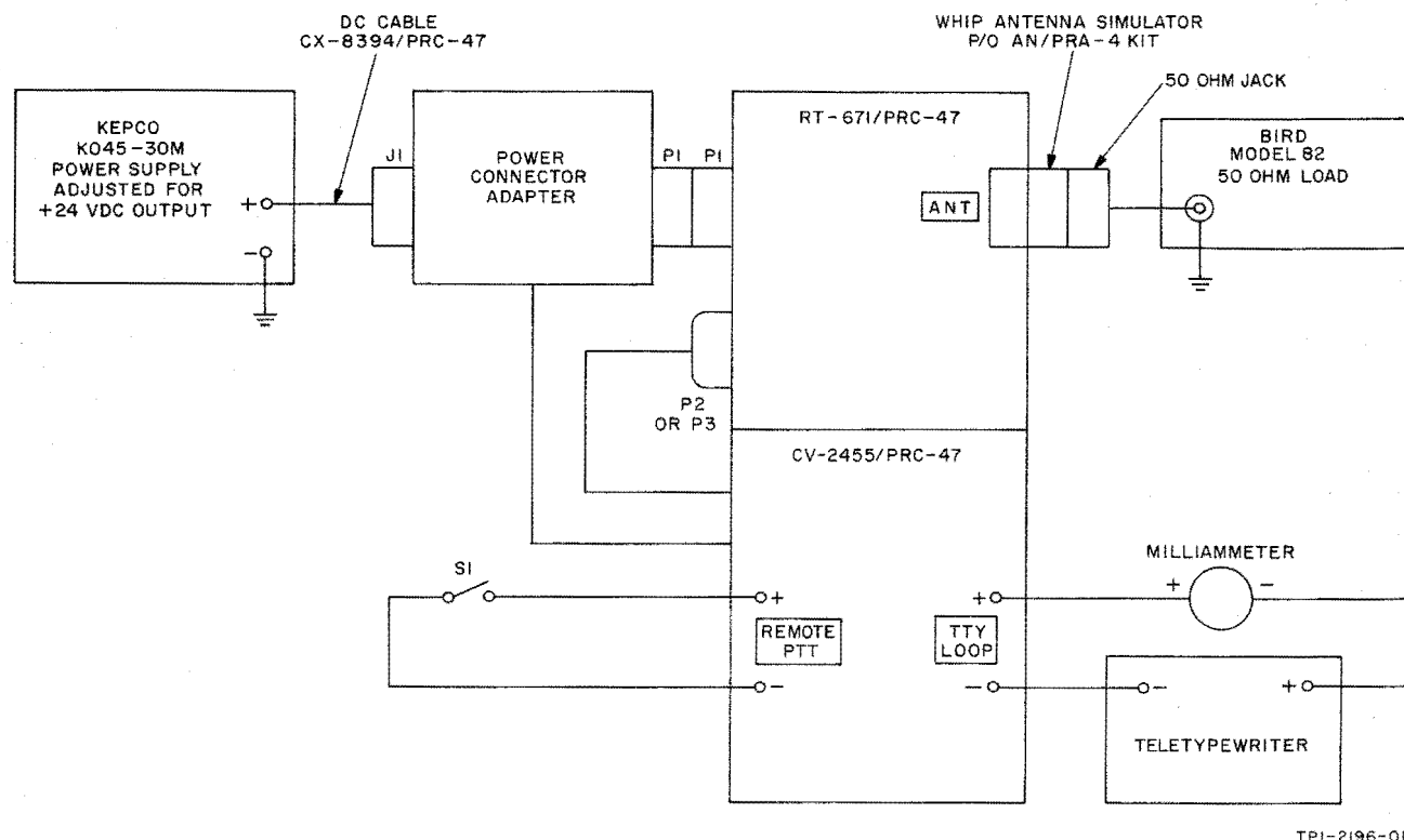
Figure 4-4. System Checkout, Test Setup
