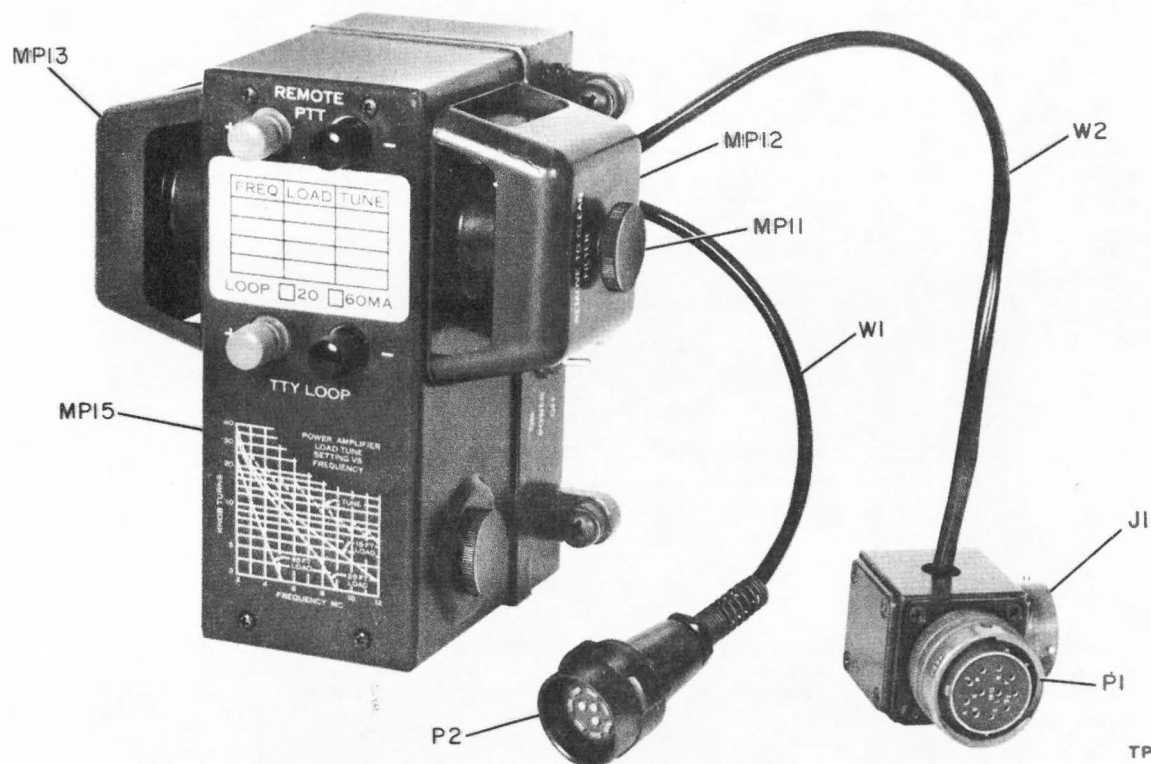
Figure 5-6. CV-2455/PRC-47, External Connection Identification
