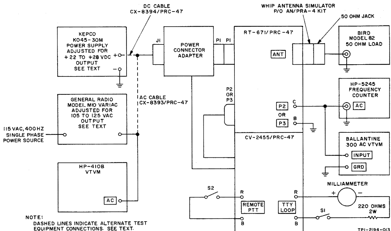
Figure 4-2. Tone Generator Operation, Test Setup
