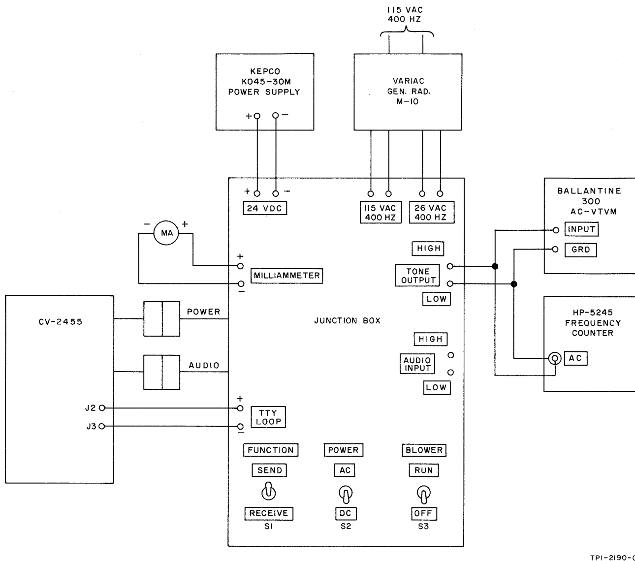
Figure 5-3. Tone Generator, Maintenance Setup
