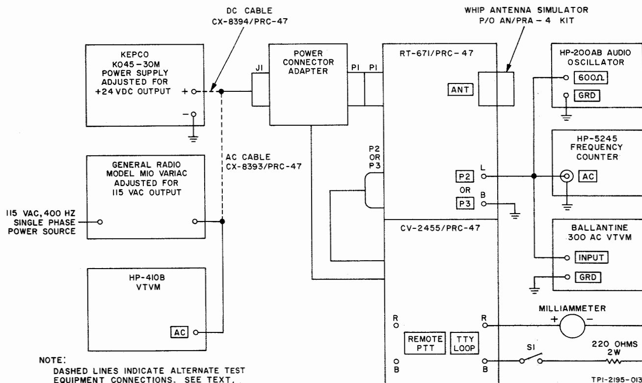
Figure 4-3. Receive Operation, Test Setup
