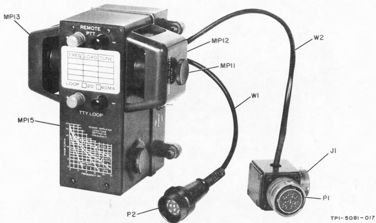
Figure 5-6. CV-2455/PRC-47, External Connection Identification
