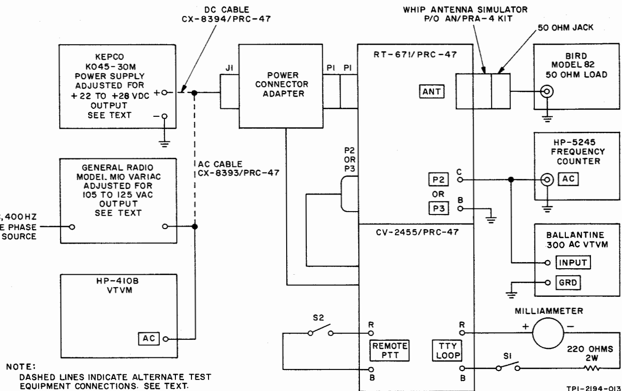
Figure 4-2. Tone Generator Operation, Test Setup
