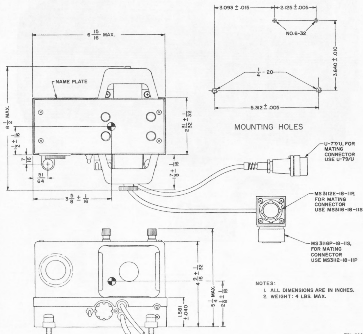
Figure 2-1. Converter-Blower CV-2455/PRC-47, Outline and Mounting Dimensions
