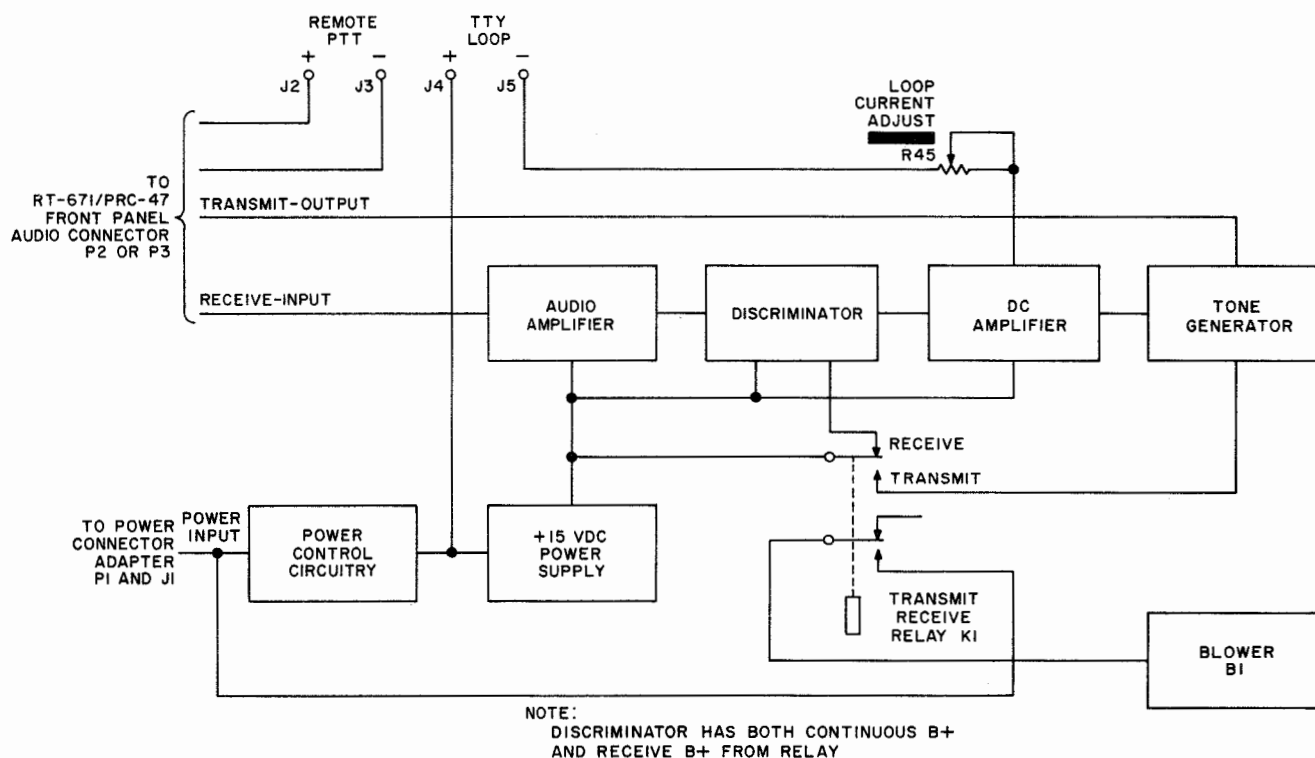
Figure 4-1. Converter-Blower CV-2455/PRC-47, Functional Block Diagram
