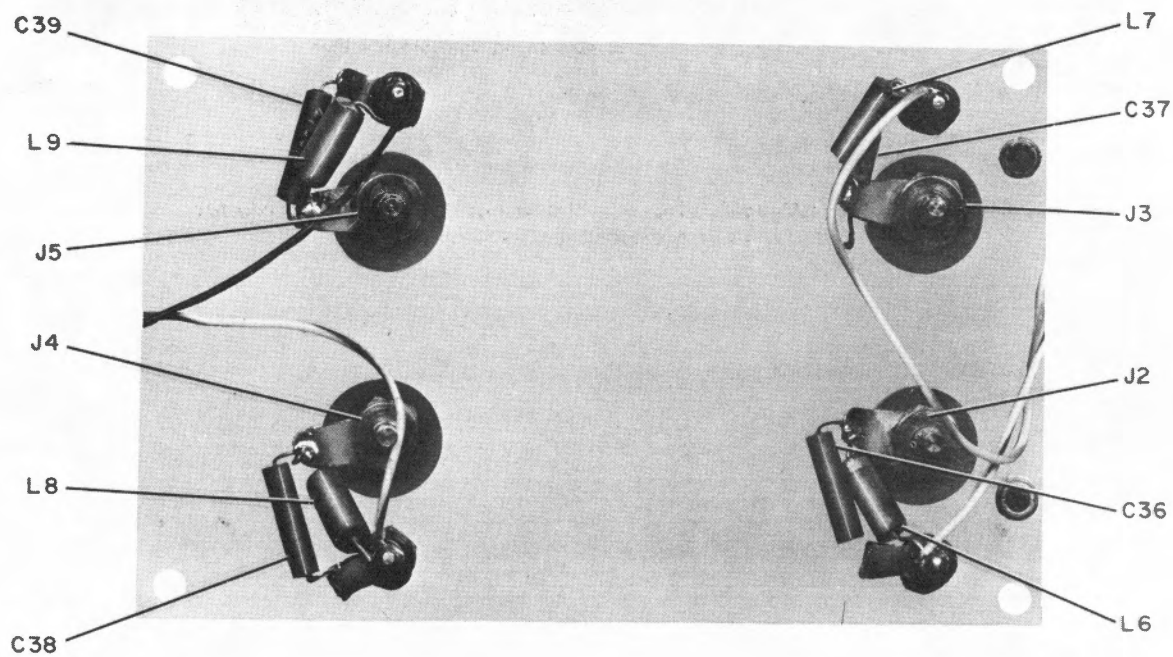
Figure 5-12. Terminal Post Support, Rear View, Chassis, Parts Location
