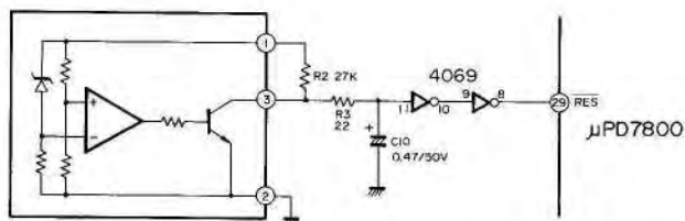
Fig. 18 Reset circuit
