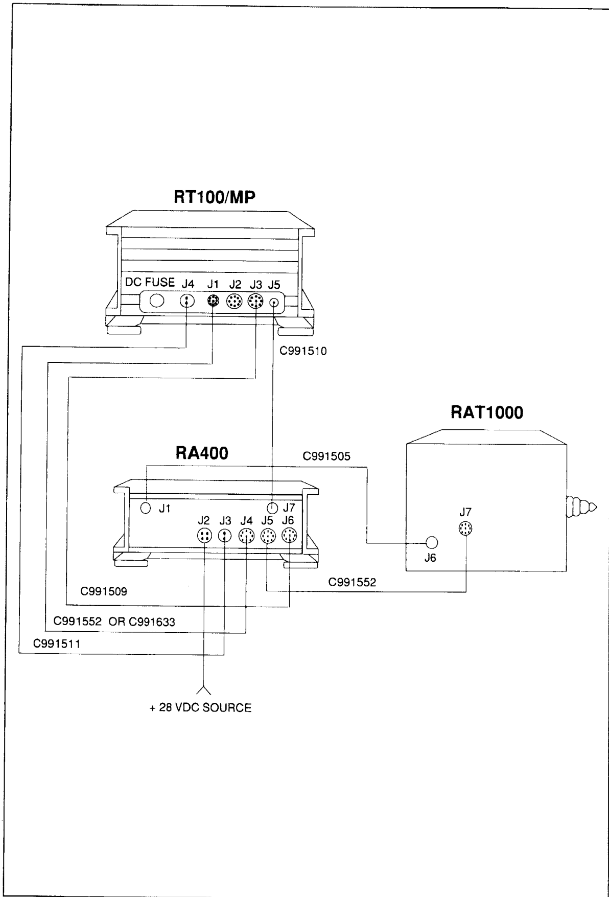
FIGURE 2-4. RT100/RA400/RAT1000 Configuration.
