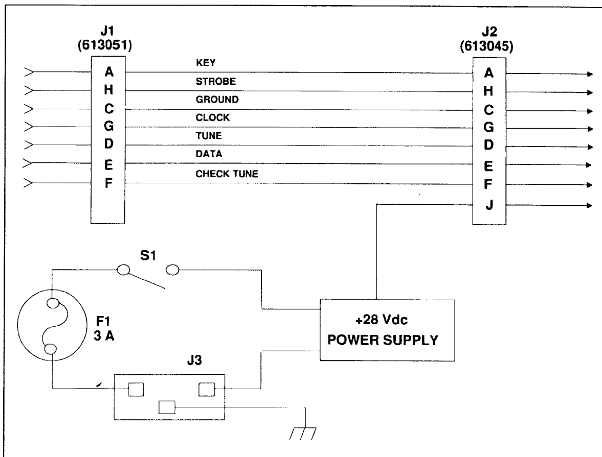
FIGURE 5-3. RAT1000P Wiring.
