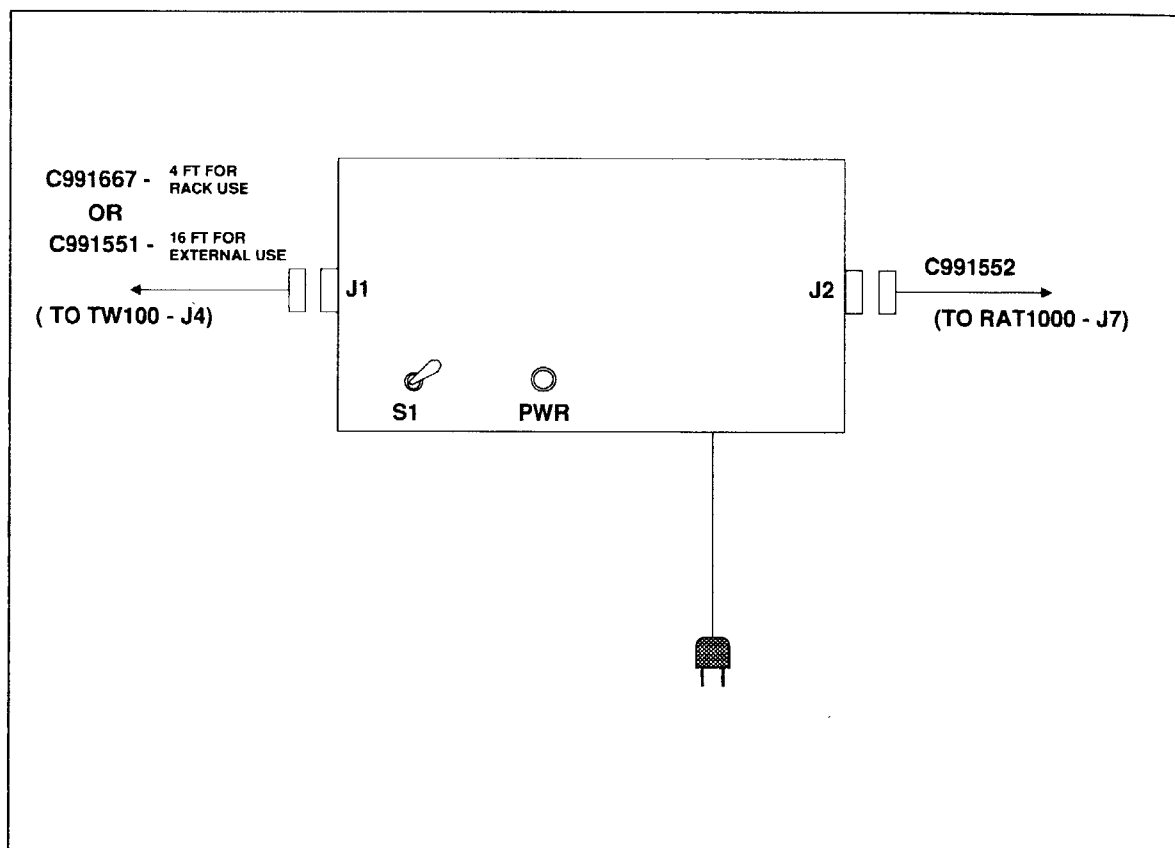
FIGURE 5-2. Block Diagram.
