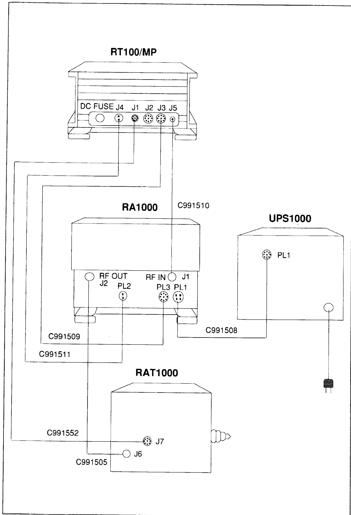
FIGURE 2-6. RT100/RA1000/RAT1000 Configuration.
