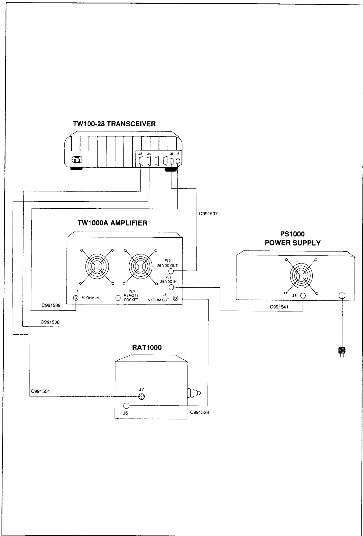
FIGURE 2-2. TW100/TW1000A/RAT1000 Configuration.
