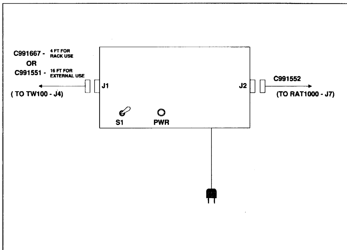
FIGURE 5-2. Block Diagram.
