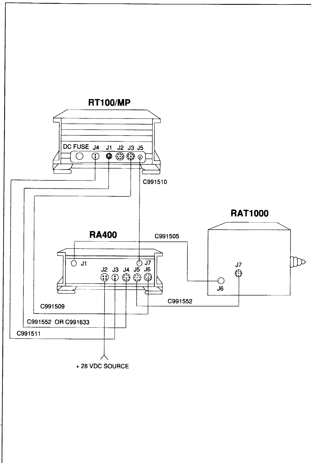
FIGURE 2-4. RT100/RA400/RAT1000 Configuration.
