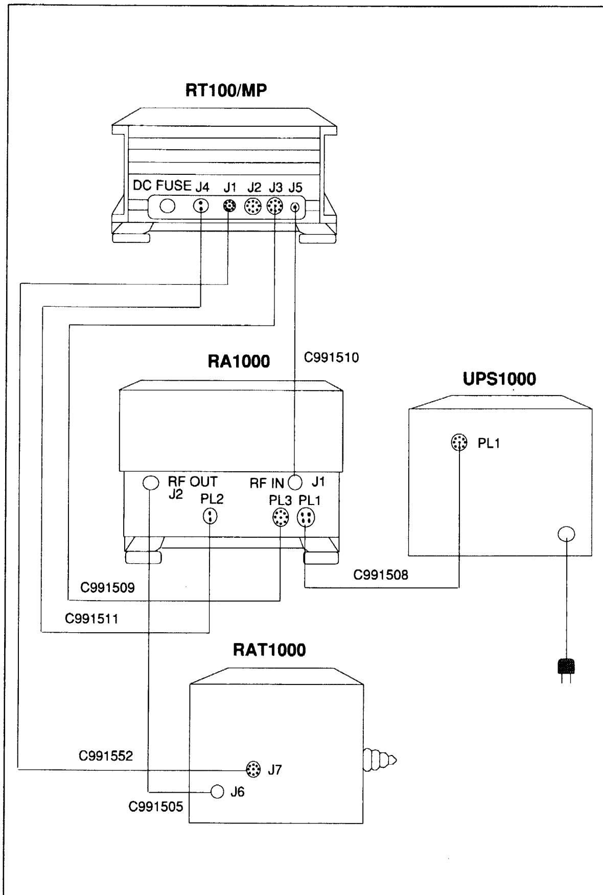
FIGURE 2-6. RT100/RA1000/RAT1000 Configuration.
