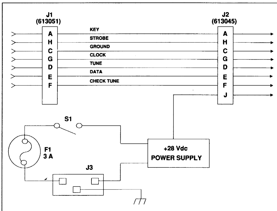
FIGURE 5-3. RAT1000P Wiring.
