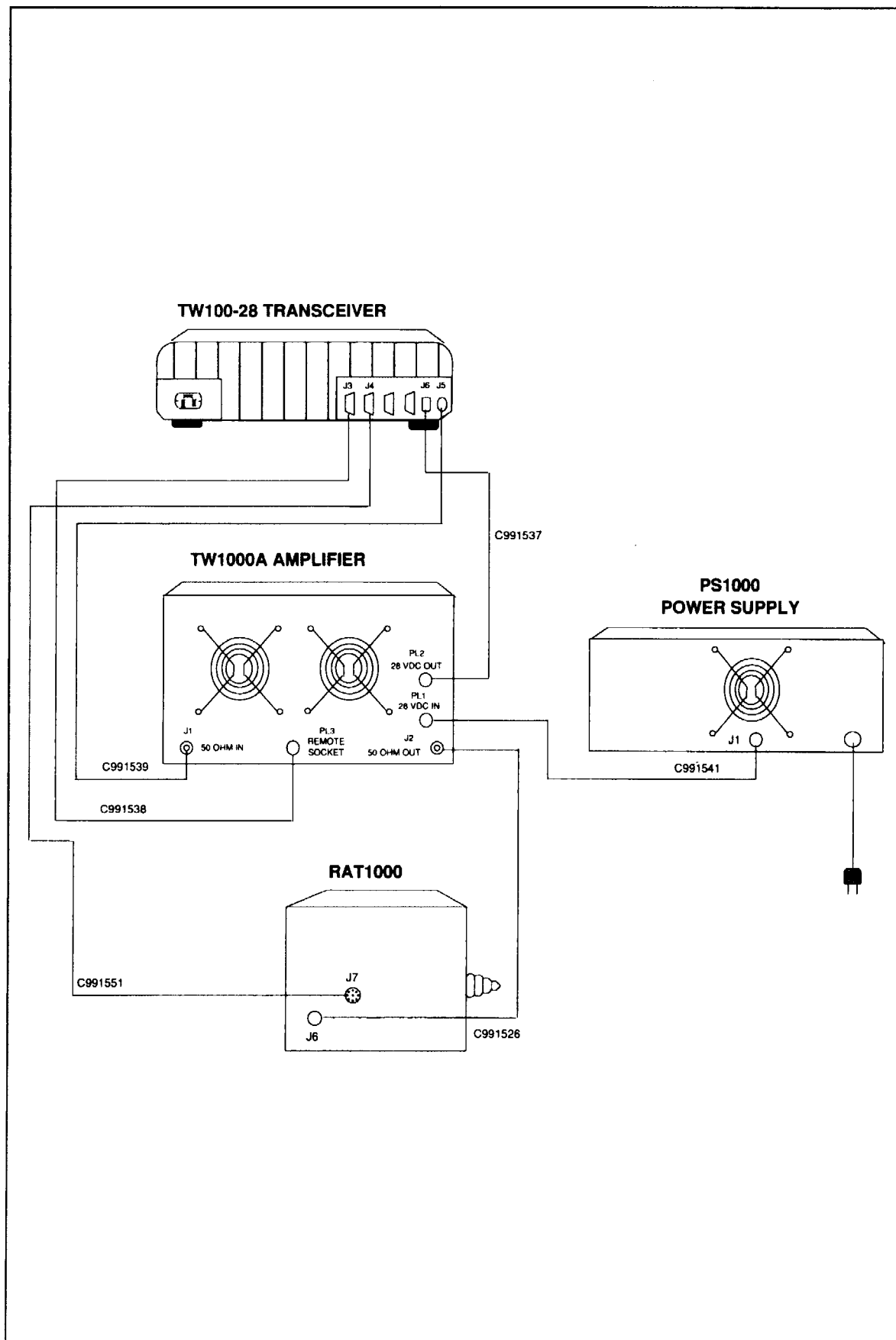
FIGURE 2-2. TW100/TW1000A/RAT1000 Configuration.
