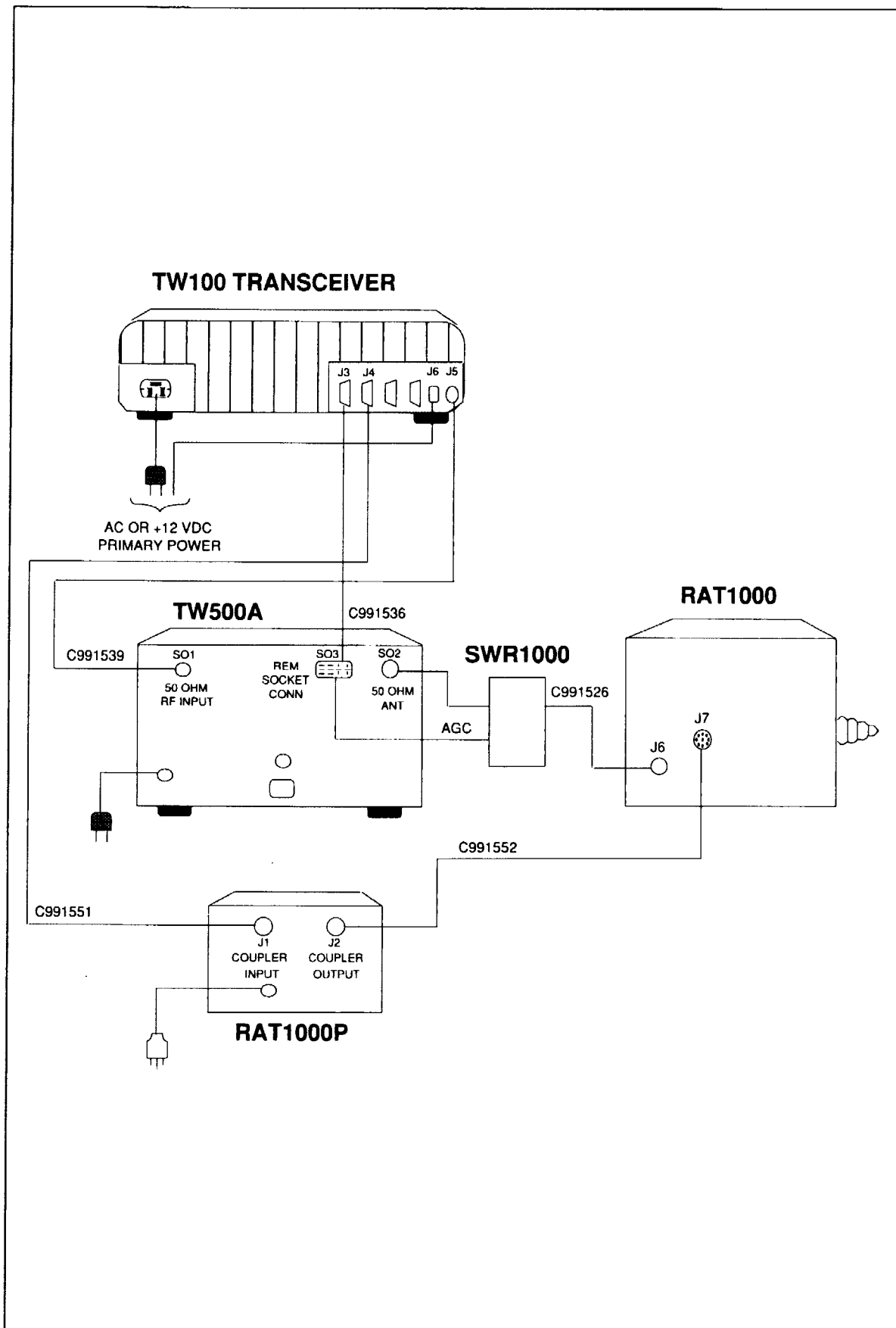
FIGURE 2-1. TW100/TW500A/RAT1000 Block Diagram.
