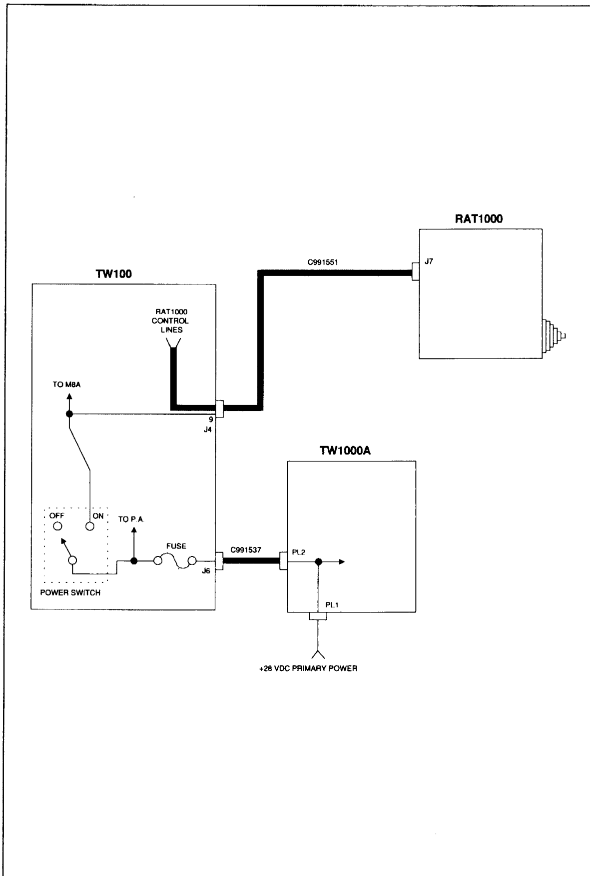
FIGURE 2-3. Primary Power Routing for Standard TW100/TW1000A/RAT1000 System.
