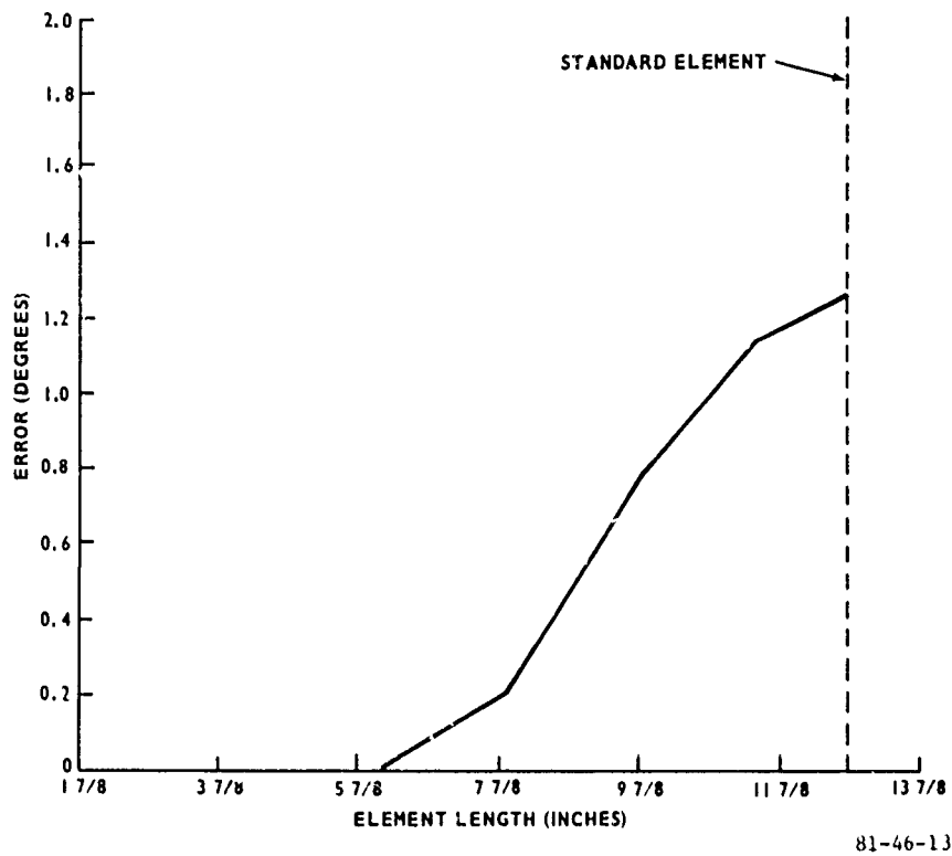
FIGURE 13. MAXIMUM ABSOLUTE BEARING ERROR VERSUS FIELD DETECTOR ELEMENT LENGTH — FIELD DETECTOR MOUNTED AT 22.5° INTERVALS AROUND THE COUNTERPOISE EDGE, 32-FOOT DIAMETER COUNTERPOISE, CALVERTON, NEW YORK
