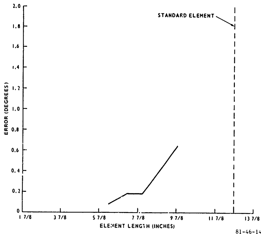
FIGURE 14. MAXIMUM ABSOLUTE BEARING ERROR VERSUS FIELD DETECTOR ELEMENT LENGTH — FIELD DETECTOR MOUNTED AT 22.5° INTERVALS AROUND THE COUNTERPOISE EDGE, 52-FOOT DIAMETER COUNTERPOISE, SALISBURY, MARYLAND
