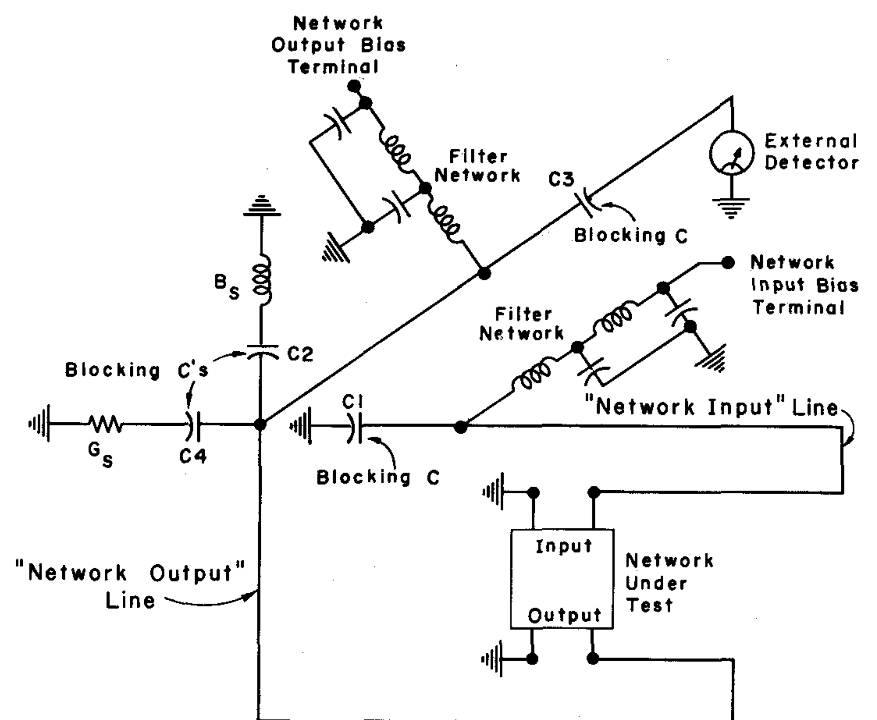
Figure 16c. Schematic diagram of dc bias circuits of the Transfer-Function and Immittance Bridge.
