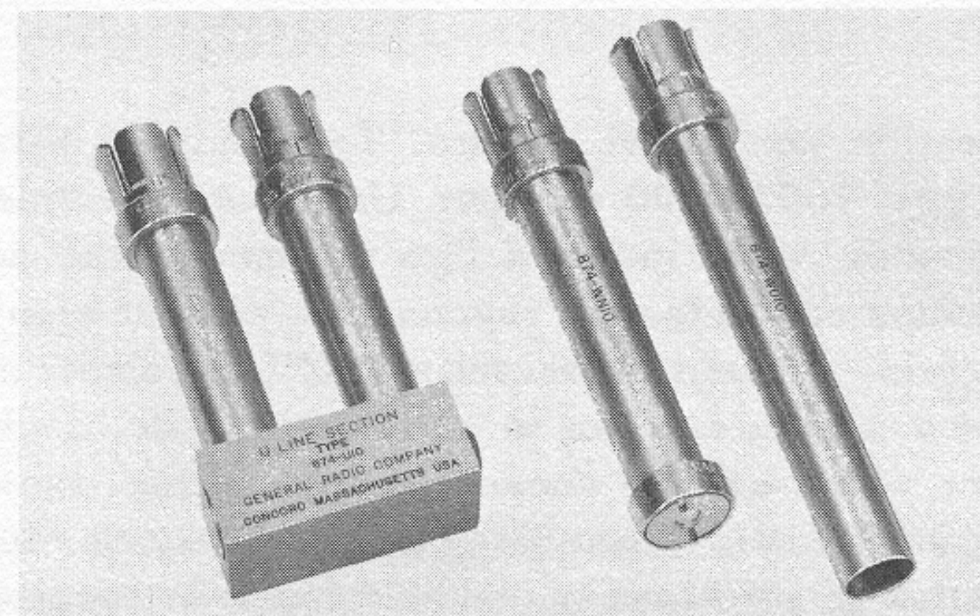
Type 1607-P40 Termination Kit.
