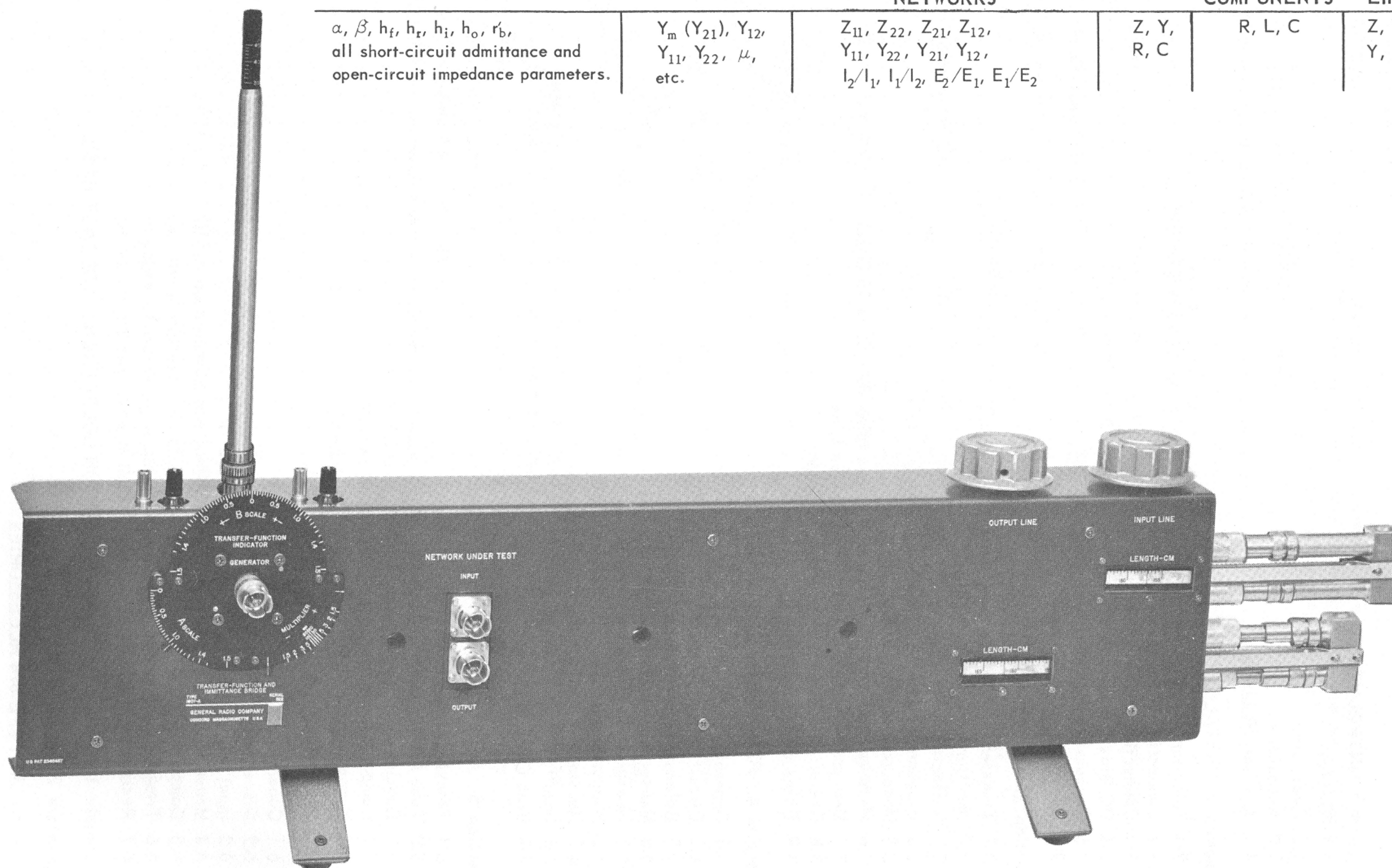
Figure 1. Type 1607-A Transfer-Function and Immittance Bridge.
