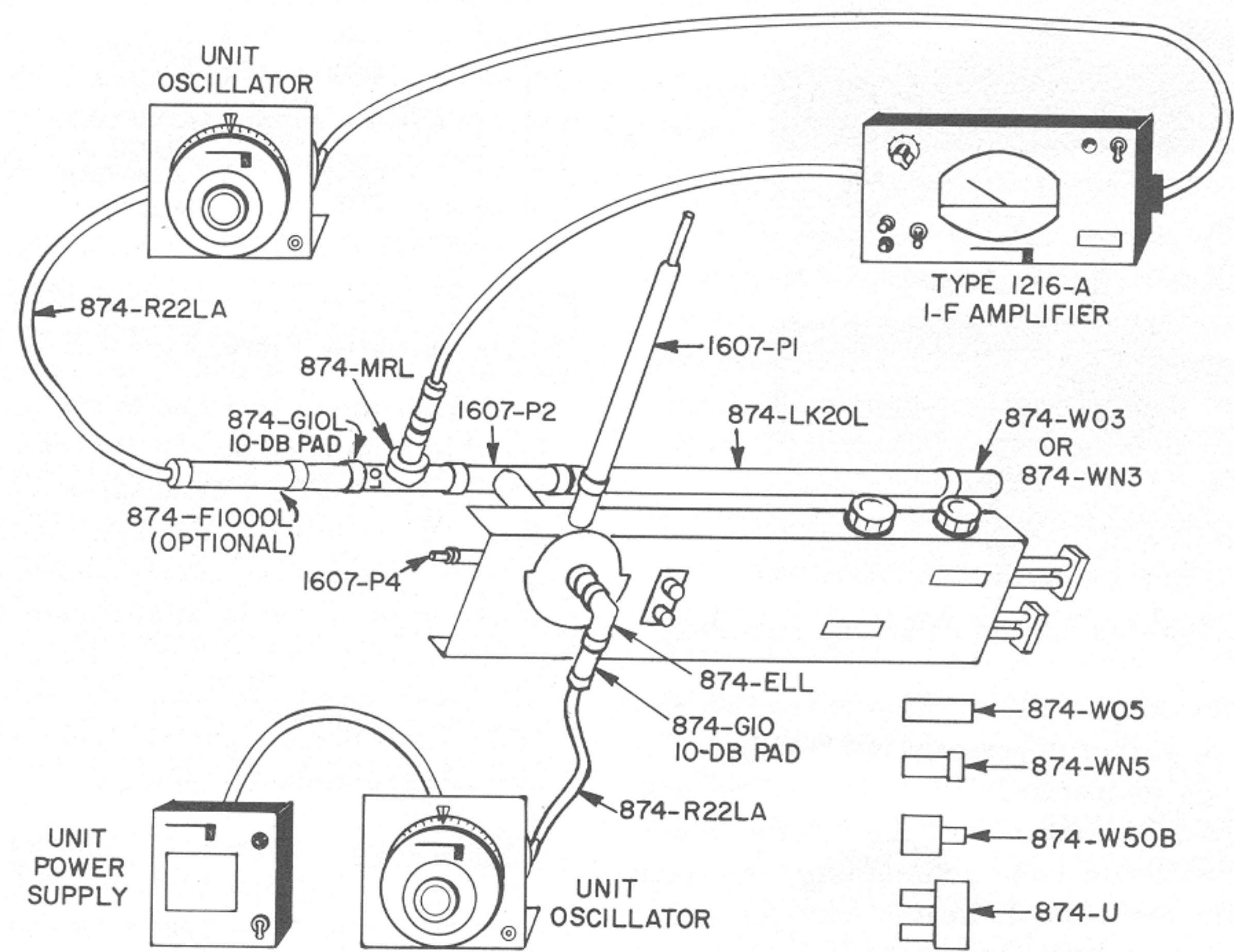
Figure 3. Typical Measurement Setup.
