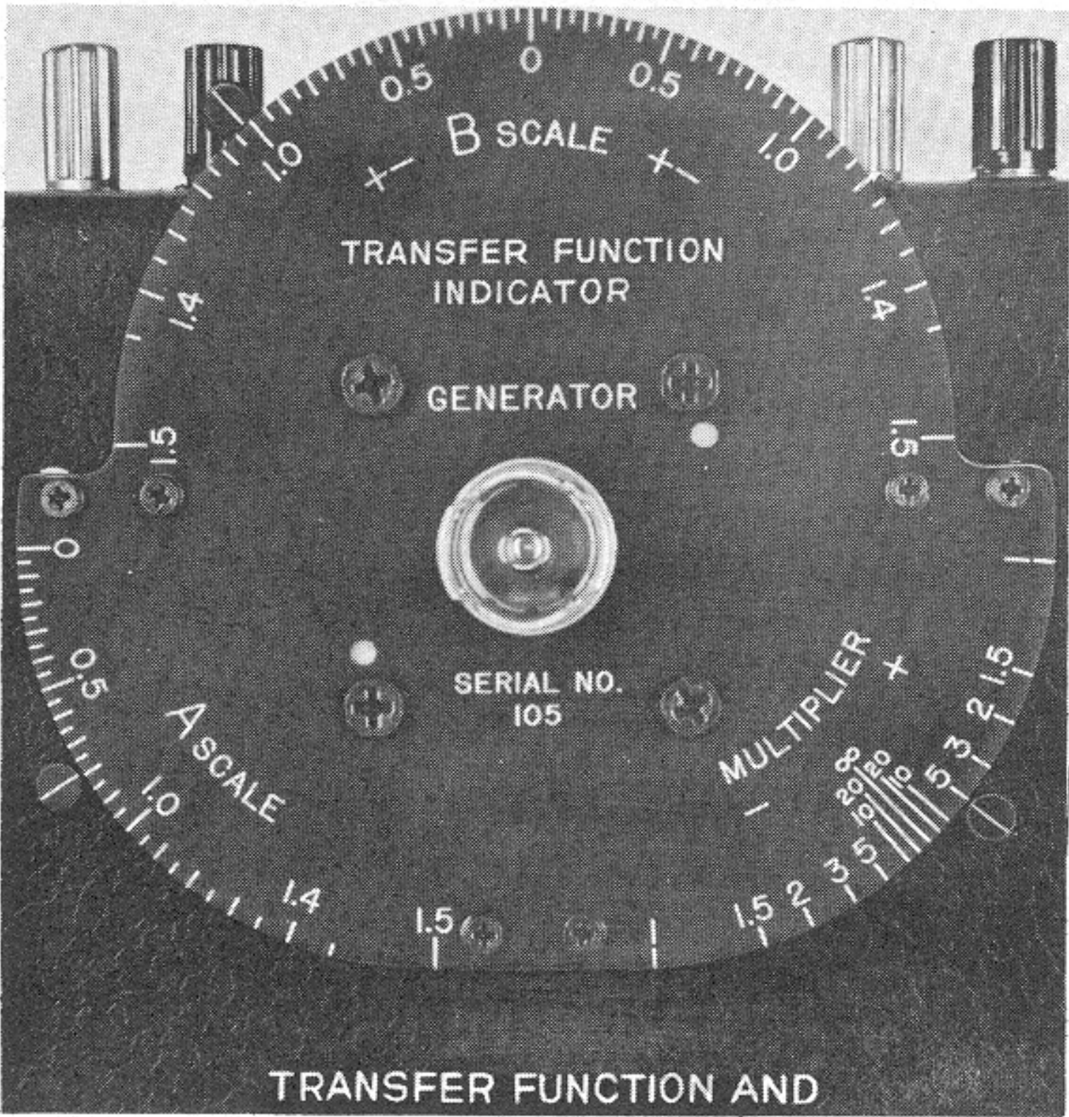
Figure 4. Transfer-Function Indicator.
