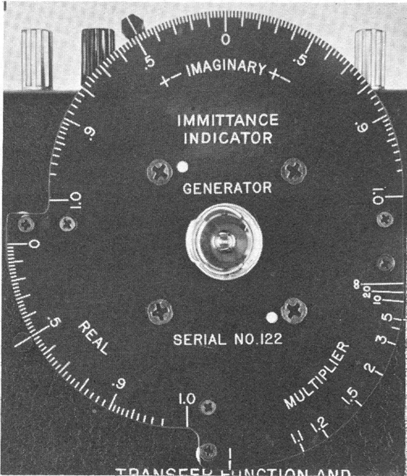
Figure 5. Immittance Indicator.
