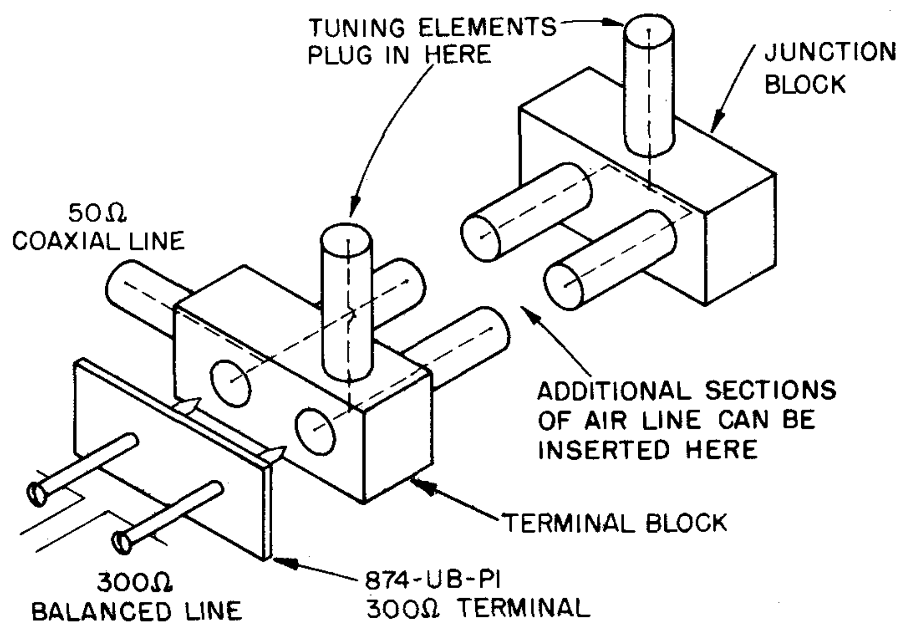
Figure 13. Functional Arrangement of Balun.
