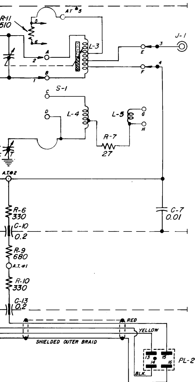
Diagram, Type 1211-B Unit Oscillator.
