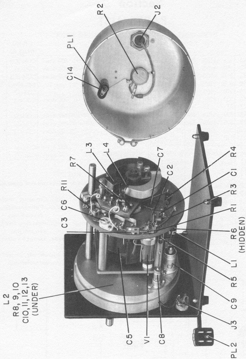
Figure 3. Interior View, Type 1211-B Unit Oscillator.
