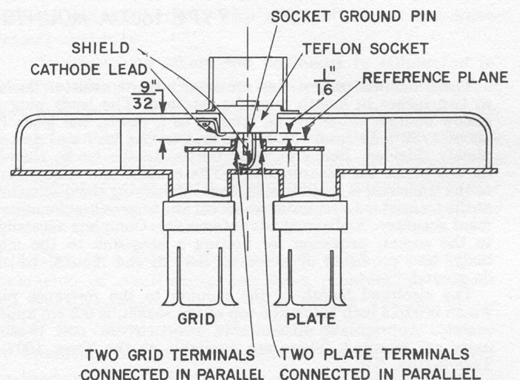
Figure 2. Mechanical Details of Tube Mount.
