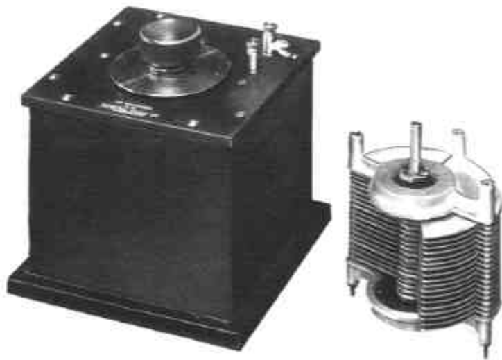
The Type 101L Variable Air Condenser, from Catalogue A.
