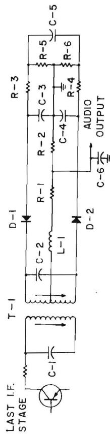
Fig. 9—Typical Ratio Detector Circuit.
