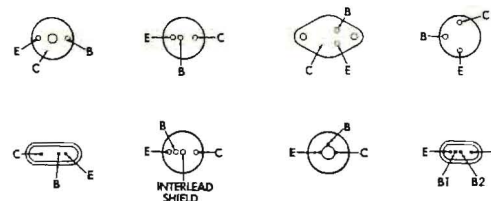
Fig. 7A—Transistor Basing Configurations.
