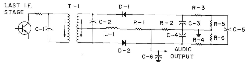
Fig. 9—Typical Ratio Detector Circuit.
